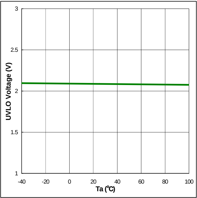
Figure 5-6. UVLO - Temperature
