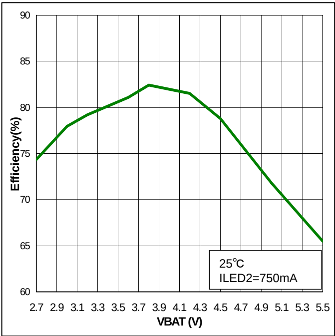
Figure 5-5. Efficiency - VBAT
