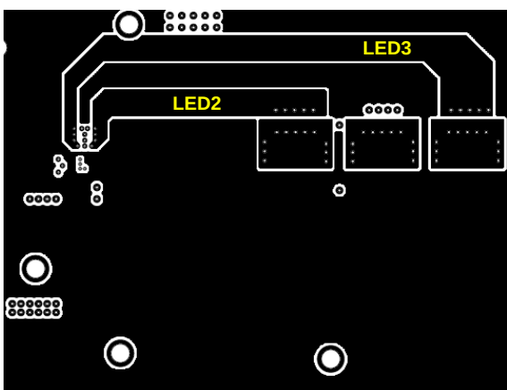
Figure 31. Middle surface2 (TOP VIEW)
