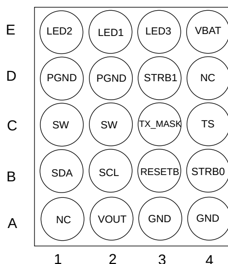
Figure 2. Pin Configuration
