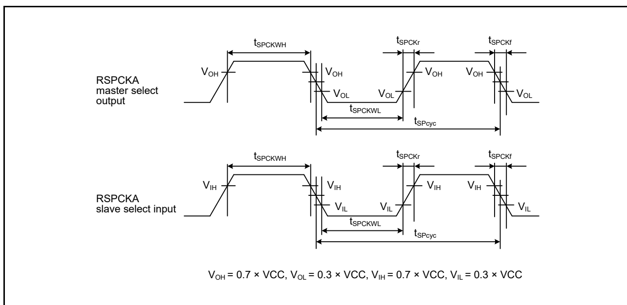
Figure 2.63 RSPI Clock Timing
