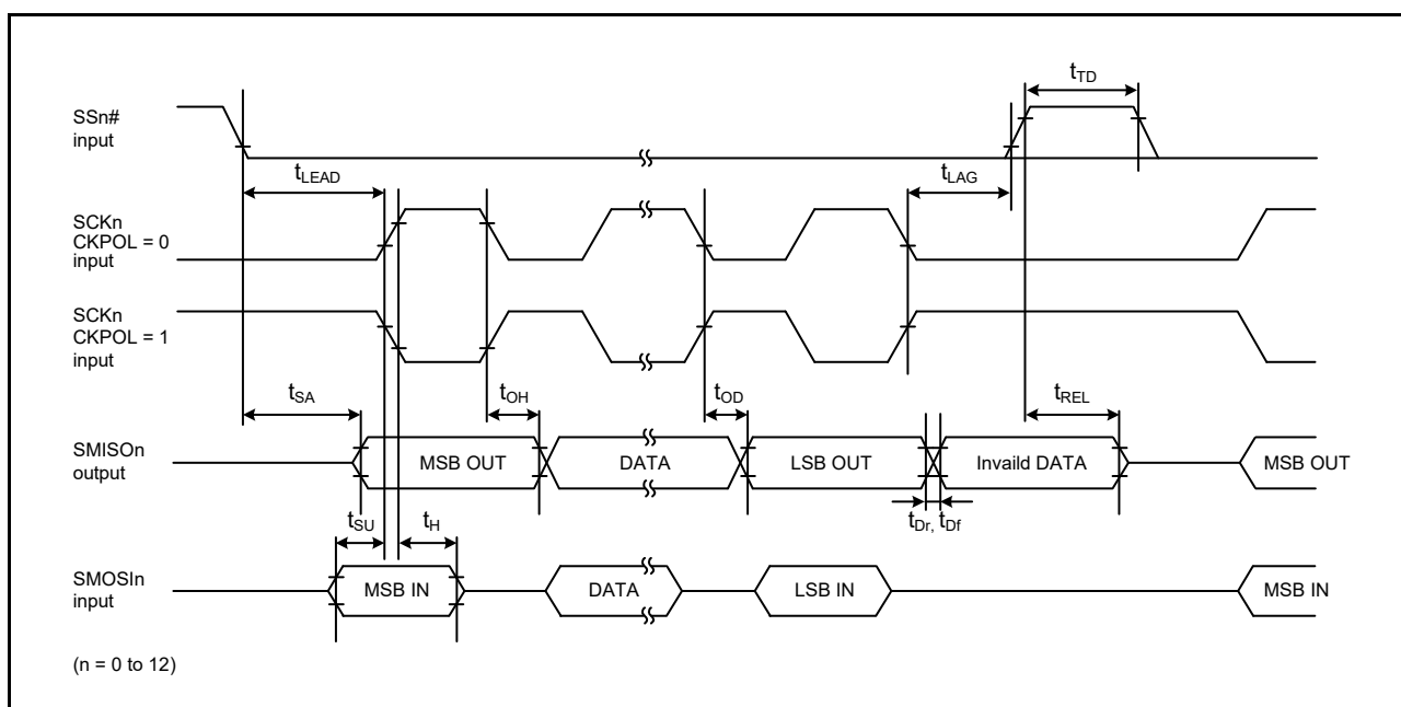
Figure 2.60 Simple SPI Timing (Slave, CKPH = 1)
