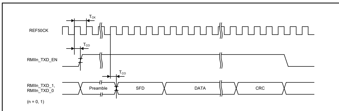
Figure 2.86 RMII Transmission Timing
