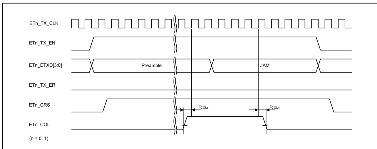
Figure 2.91 MII Transmission Timing (Conflict Occurrence)
