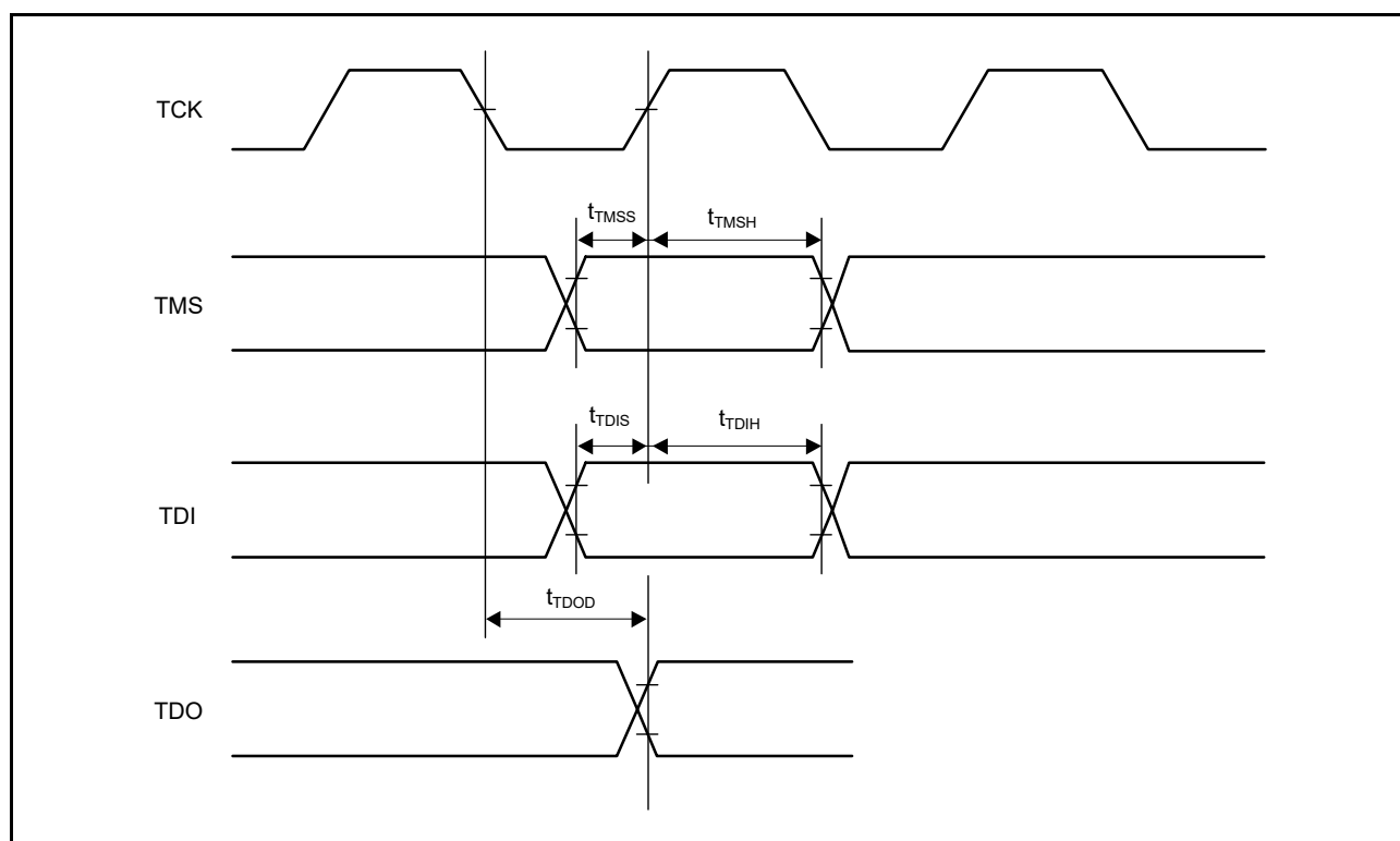
Figure 2.118 Boundary Scan Input/Output Timing
