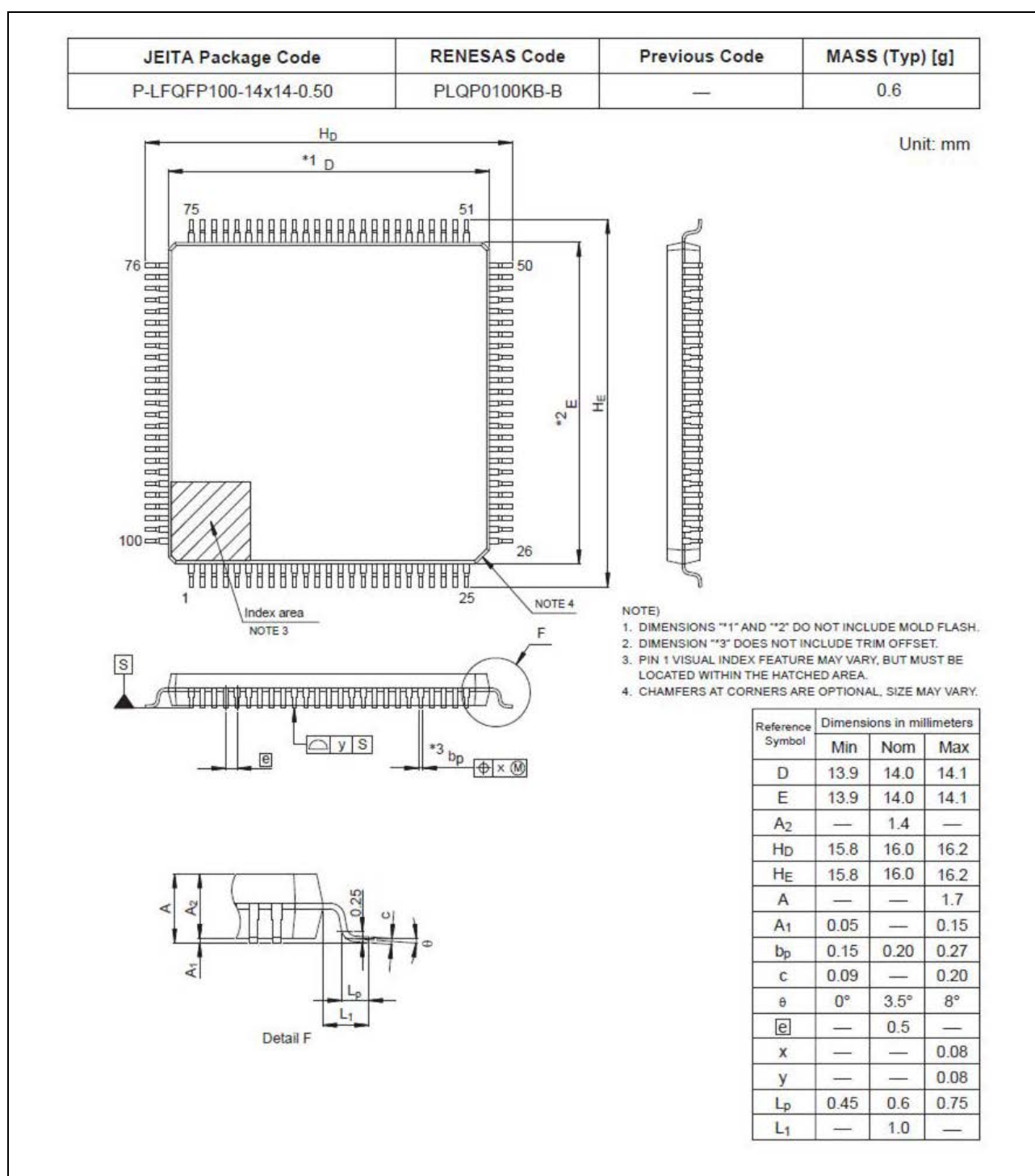
Figure E 100-Pin LFQFP (PLQP0100KB-B)
