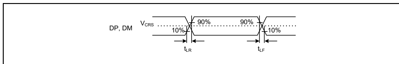
Figure 2.105 DP and DM Output Timing (Low Speed)
