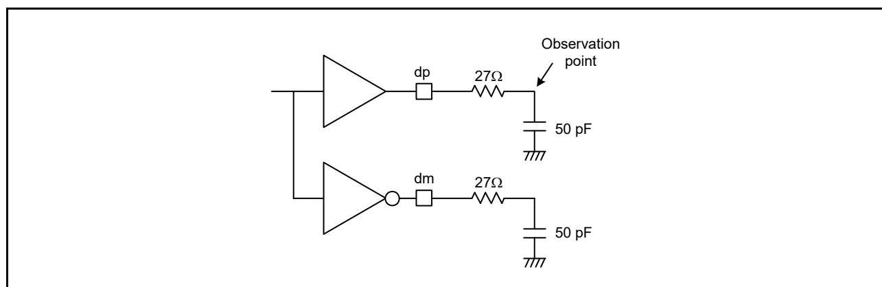
Figure 2.108 Test Circuit (Full-Speed)
