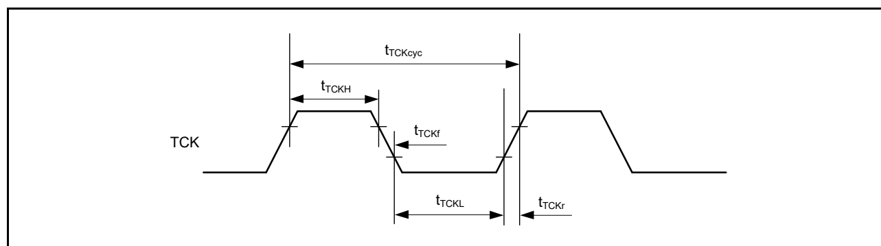
Figure 2.116 Boundary Scan TCK Timing
