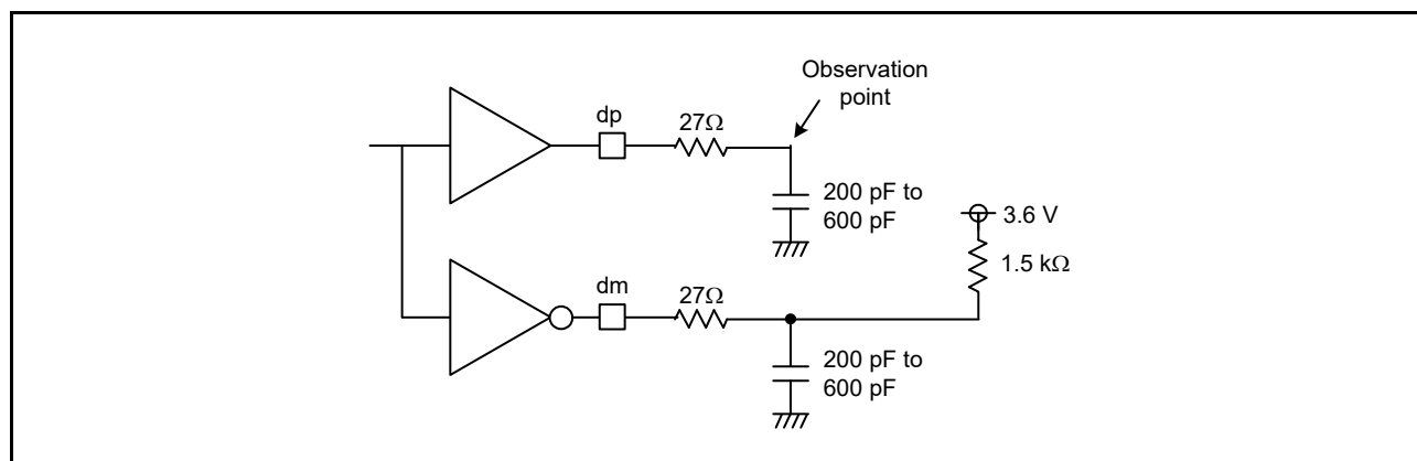
Figure 2.106 Test Circuit (Low Speed)
