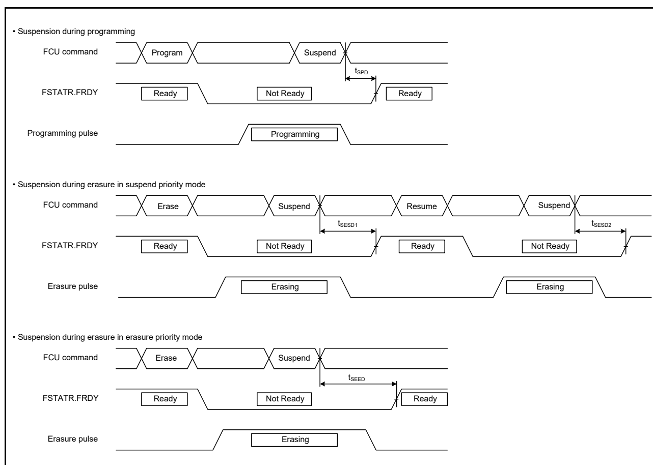
Figure 2.115 Flash Memory Programming/Erasure Suspension Timing
