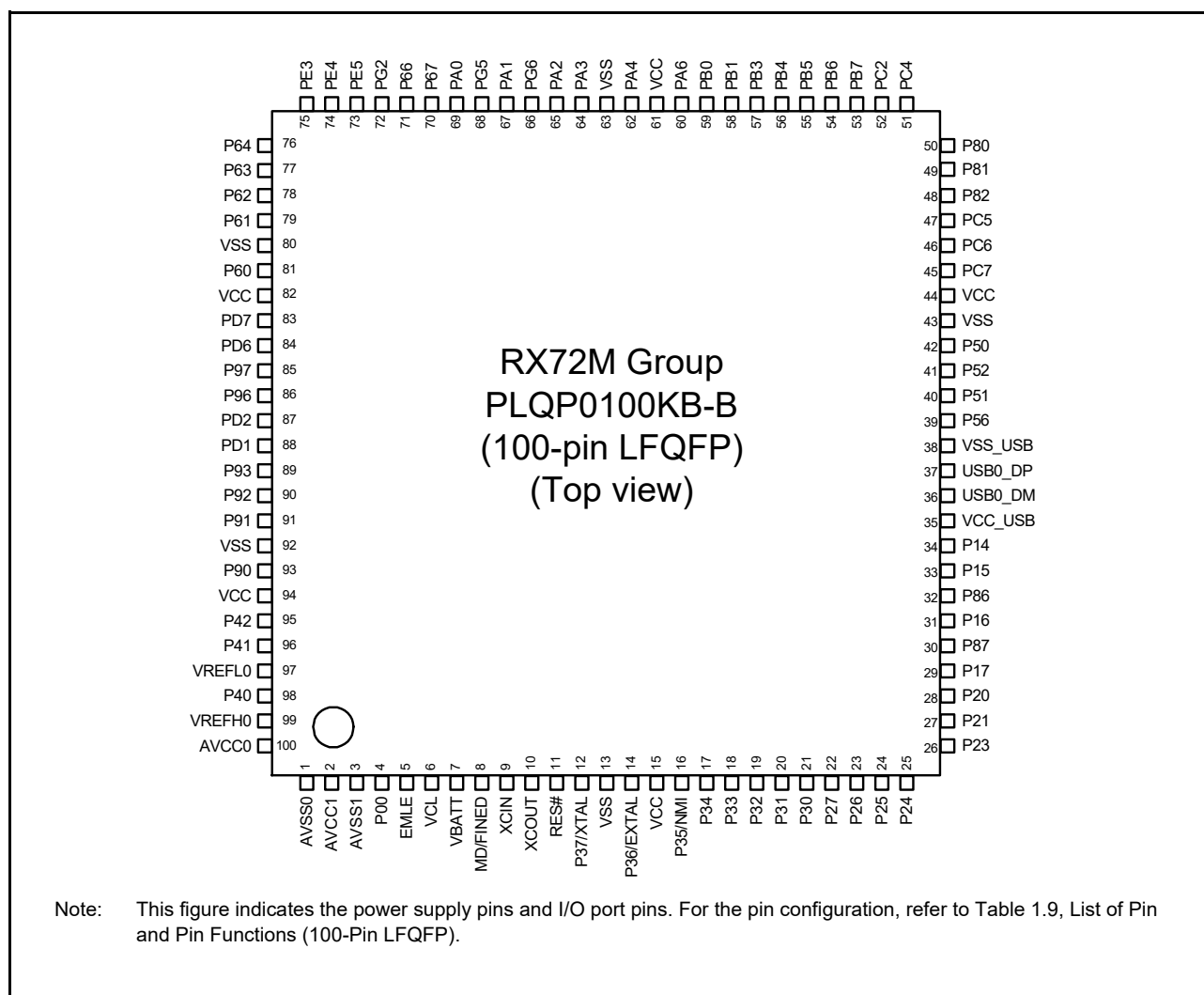
Figure 1.7 Pin Assignment (100-Pin LFQFP)
