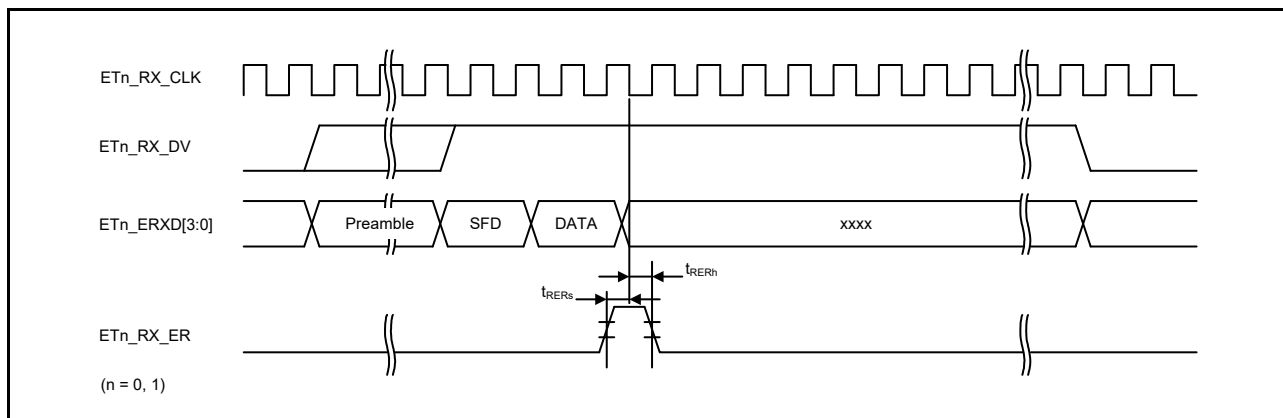
Figure 2.93 MII Reception Timing (Error Occurrence)
