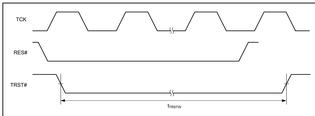
Figure 2.117 Boundary Scan TRST# Timing
