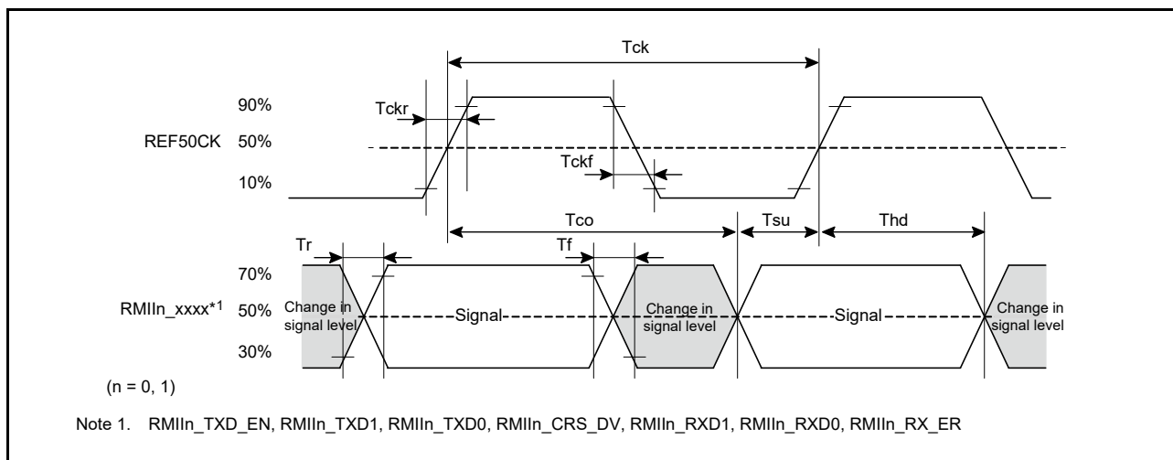
Figure 2.85 Timing with the REF50CK and RMII Signals
