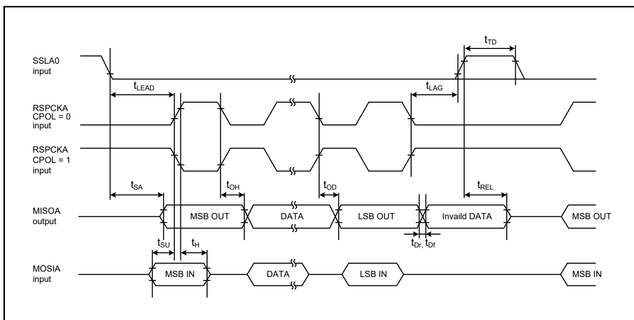
Figure 2.68 RSPI Timing (Slave, CPHA = 0)
