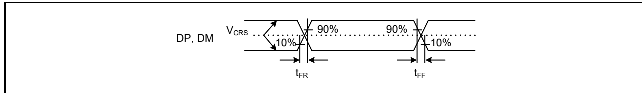
Figure 2.107 DP and DM Output Timing (Full-Speed)
