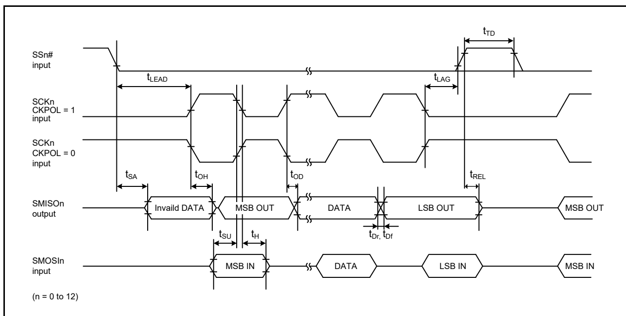
Figure 2.61 Simple SPI Timing (Slave, CKPH = 0)
