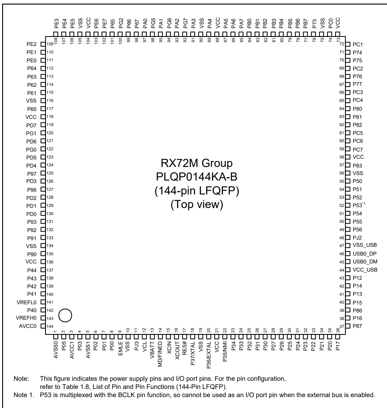
Figure 1.6 Pin Assignment (144-Pin LFQFP)
