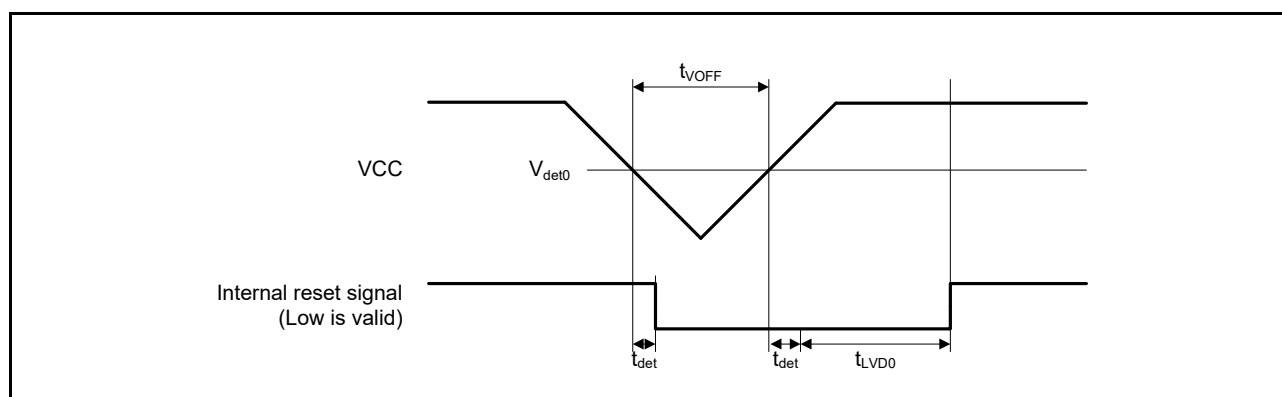
Figure 2.110 Voltage Detection Circuit Timing ( V_{det0} )
