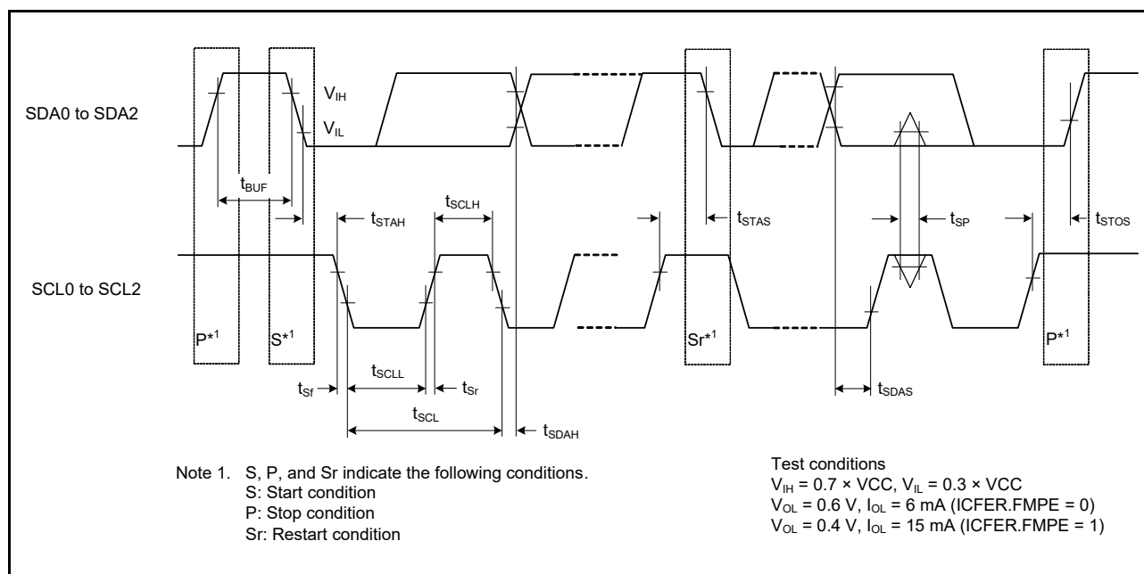
Figure 2.62 RIIC Bus Interface Input/Output Timing
