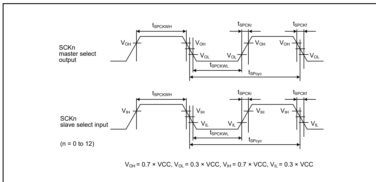
Figure 2.57 Simple SPI Clock Timing
