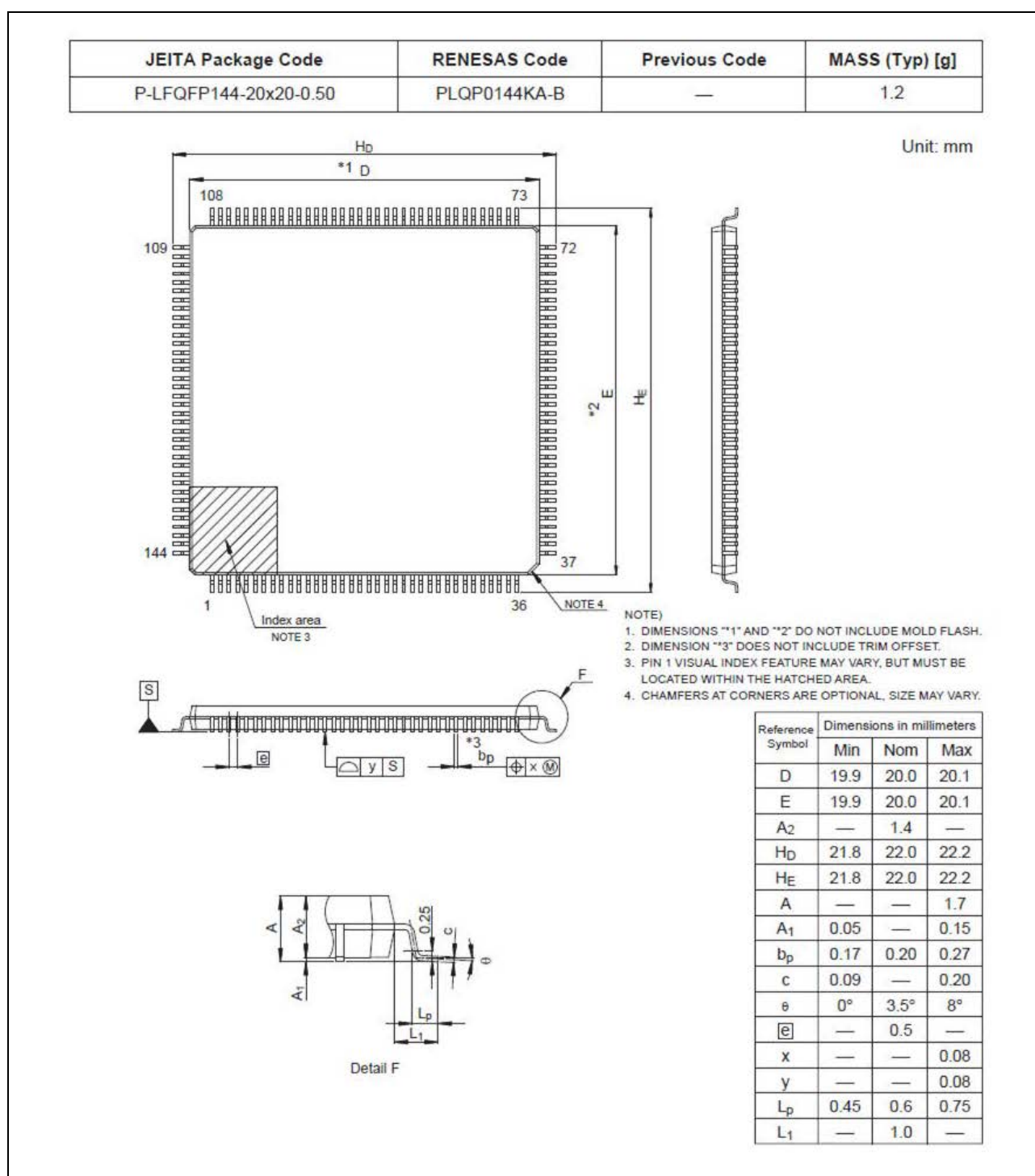
Figure D 144-Pin LFQFP (PLQP0144KA-B)
