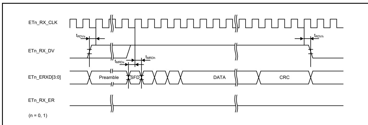
Figure 2.92 MII Reception Timing (Normal Operation)
