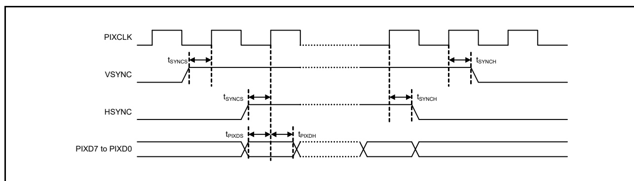
Figure 2.97 PDC AC Timing
