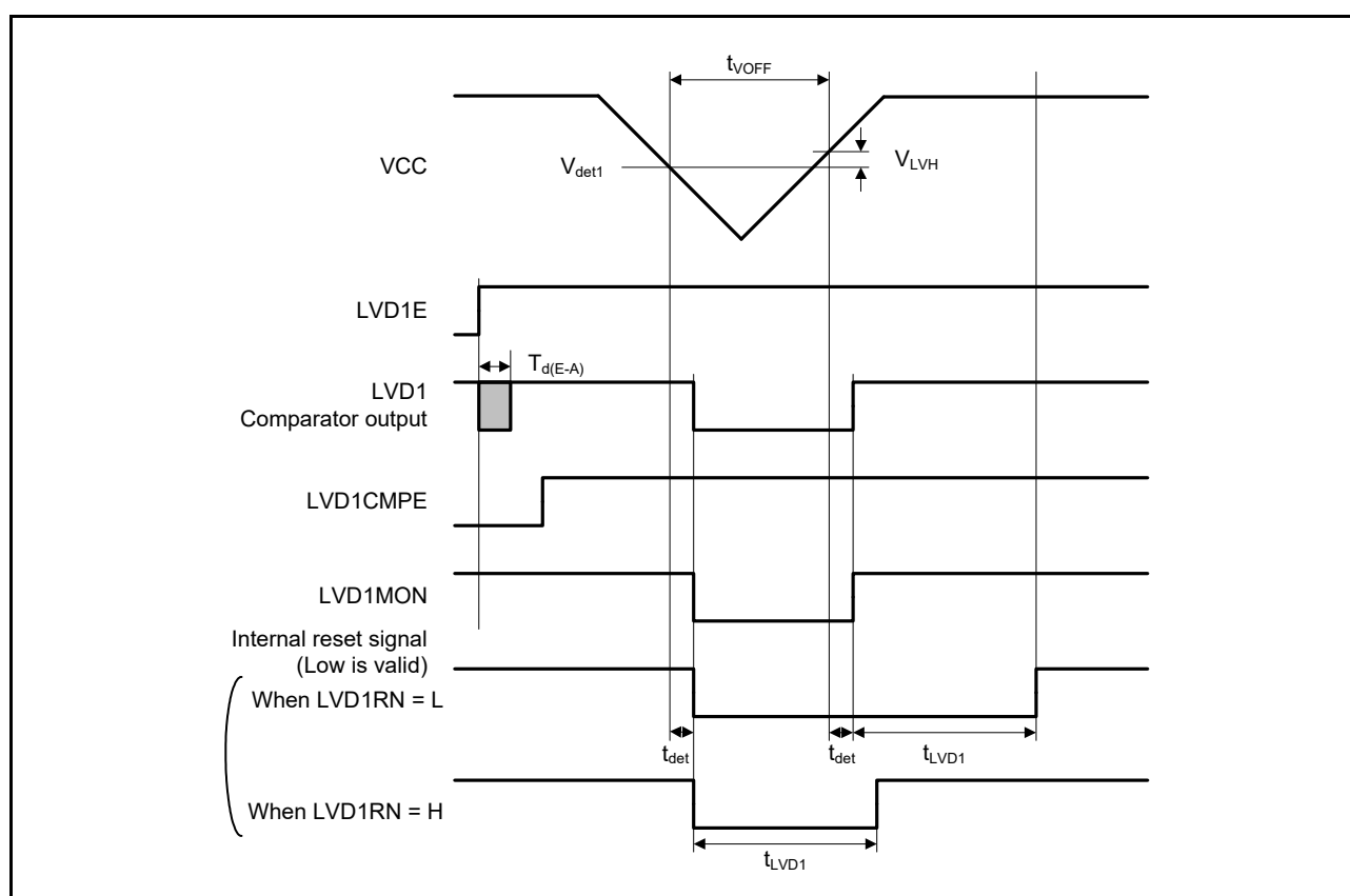
Figure 2.111 Voltage Detection Circuit Timing ( V_{det1} )
