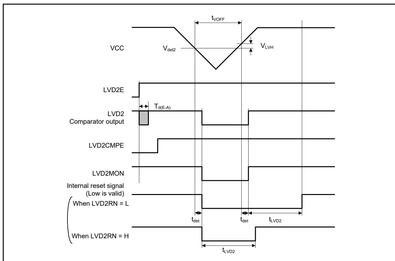
Figure 2.112 Voltage Detection Circuit Timing (V det2 )
