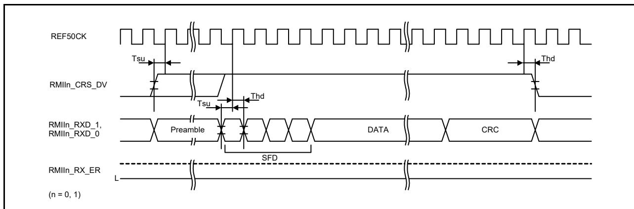
Figure 2.87 RMII Reception Timing (Normal Operation)
