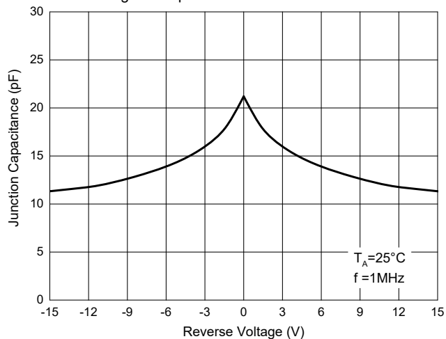
Fig. 3 - Capacitance Characteristics
