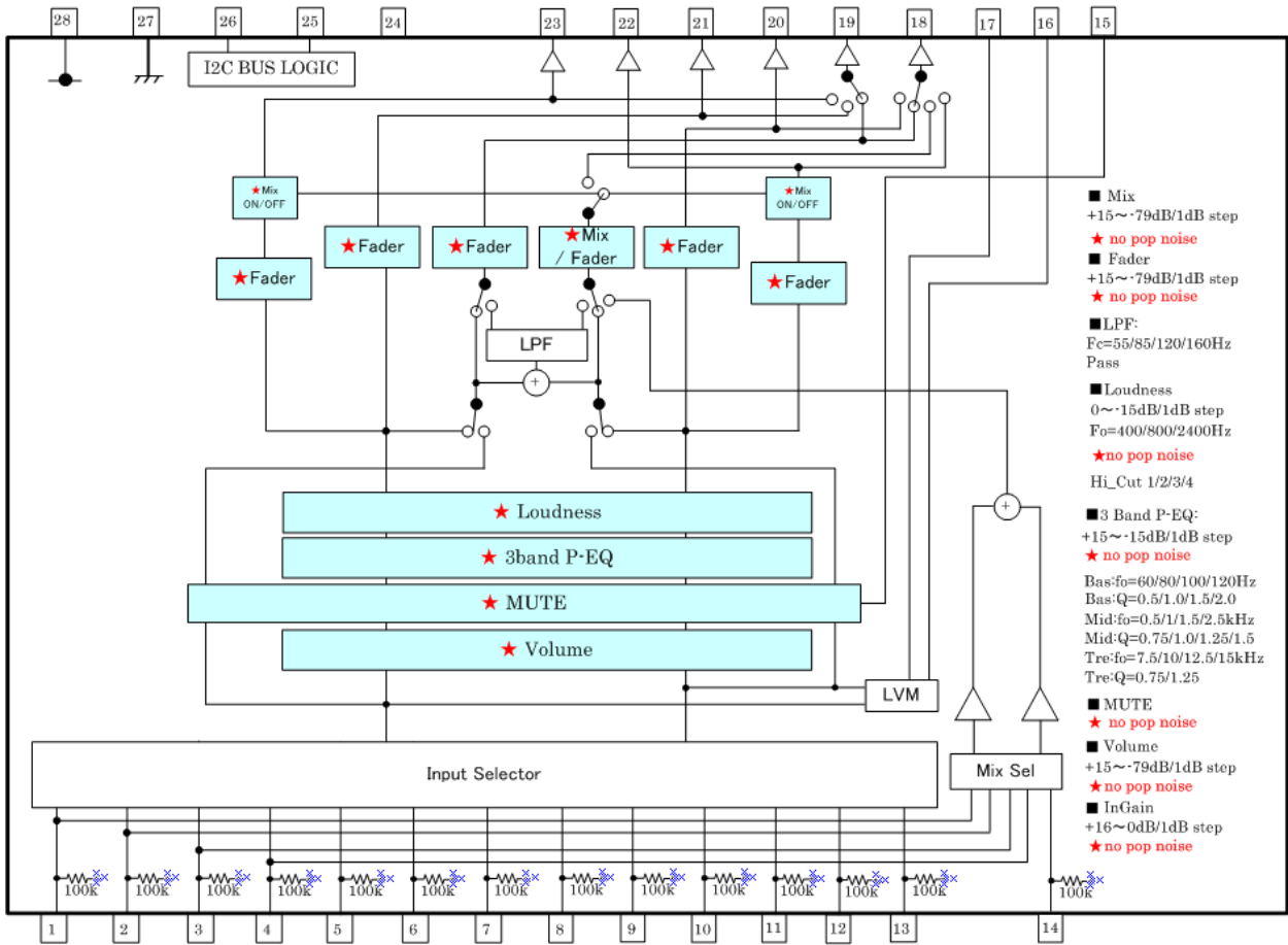
Figure 3. Block Diagram
