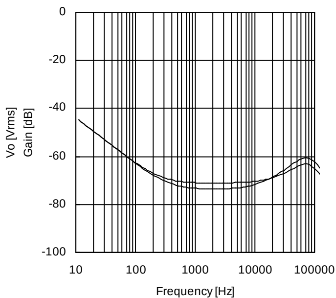
Figure 7. CMRR
