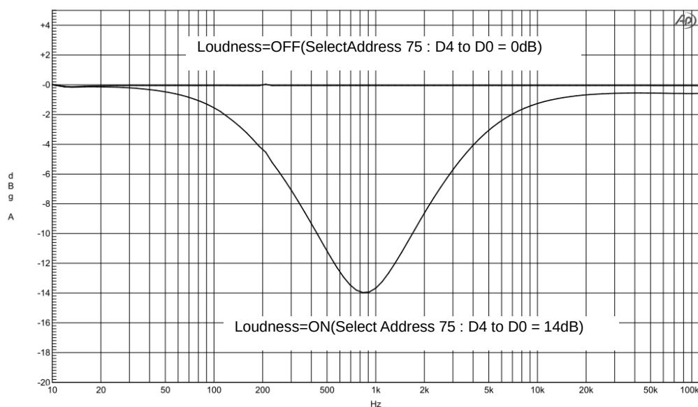
Figure 19. Loudness gain vs frequency ( f_o=800\text{Hz} )
