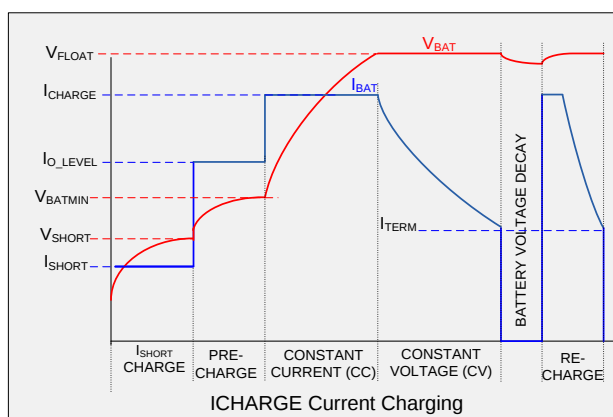
Figure 35. Charge Curve, I CHARGE Not Limited by I BUSLIM
