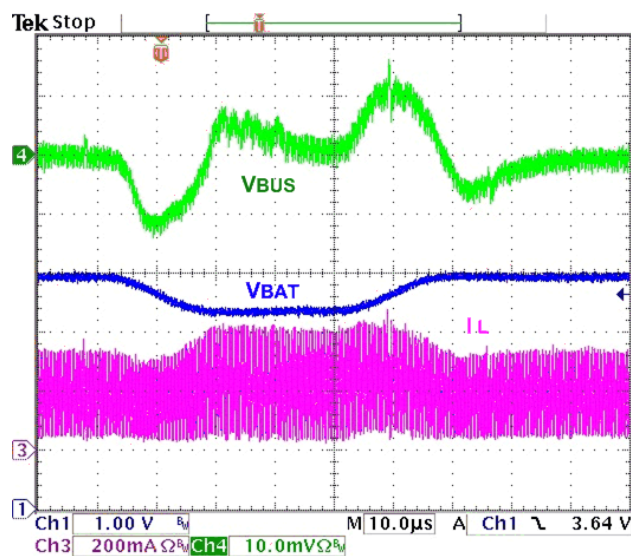
Figure 34. Line Transient, 50 \Omega Load, 3.9-3.3-3.9 V_{BAT} , t_{RISE/FALL}=10\text{ }\mu\text{s}
