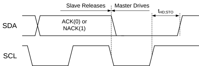
Figure 48. Stop Bit
