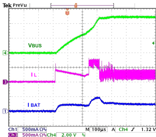
Figure 31. OTG Startup, 50 \Omega Load, 3.6 V_{BAT} External / Additional 10 \mu\text{s} on VBUS
