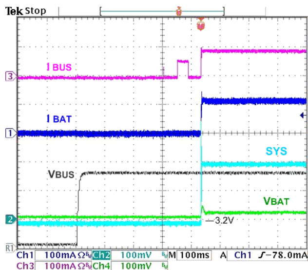
Figure 11. Charge Startup at V_{\text{BUS}} Plug-In, 100 mA I_{\text{BUSLIM}} , 3.2 V V_{\text{BAT}} , 100 \Omega SYS Load
