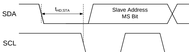
Figure 47. Start Bit
