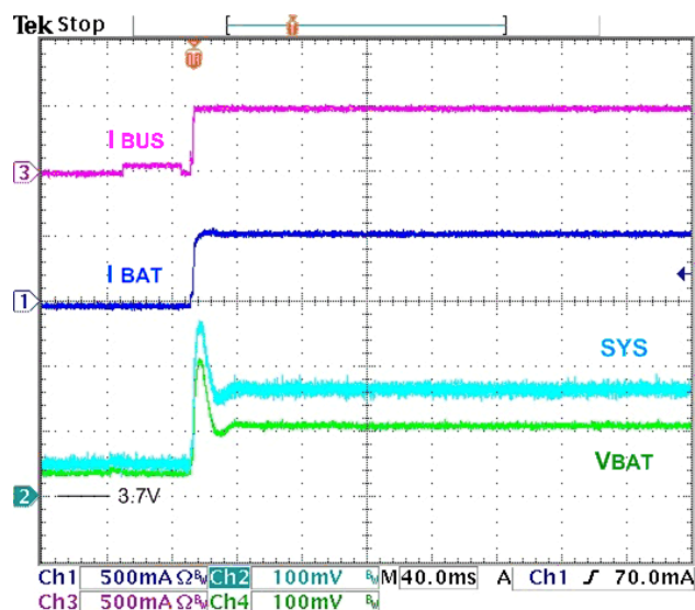
Figure 14. Charge Startup with HZ Bit Reset, 500 mA I_{\text{BUSLIM}} , 950 mA I_{\text{CHARGE}} , 50 \Omega SYS Load
