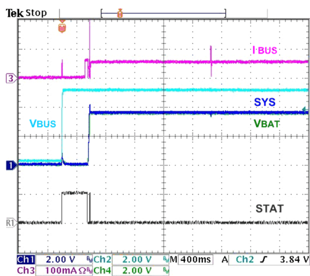
Figure 18. No Battery at V_{\text{BUS}} Power-Up, FAN54042, 100\ \Omega SYS Load, 1\text{ k}\Omega V_{\text{BAT}} Load
