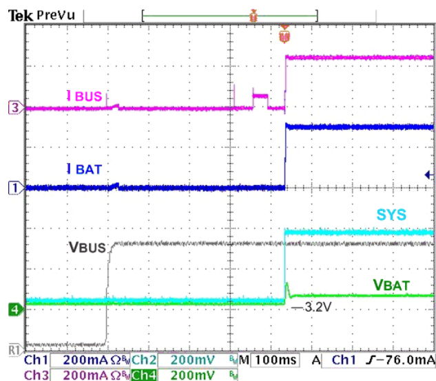
Figure 12. Charge Startup at V_{\text{BUS}} Plug-In, 500 mA I_{\text{BUSLIM}} , 3.2 V V_{\text{BAT}} , 100 \Omega SYS Load
