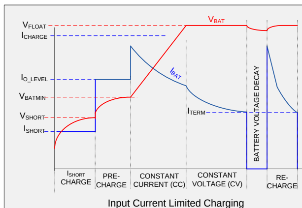
Figure 36. Charge Curve, I BUSLIM Limits I CHARGE
