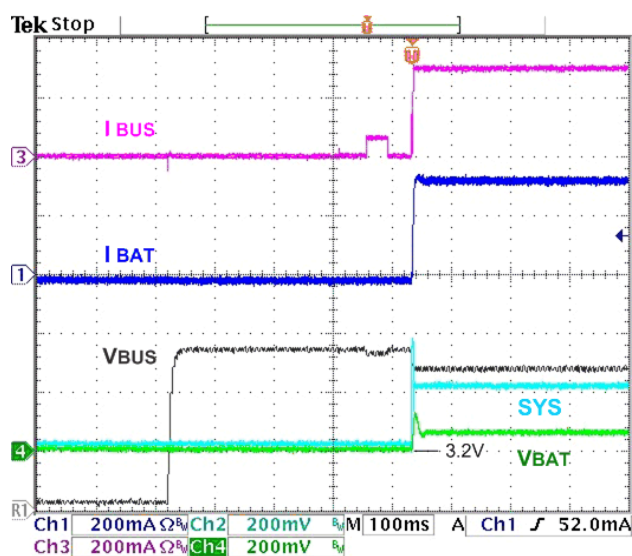
Figure 13. Charge Startup at V_{\text{BUS}} Plug-In Using 300 mA Current Limited Source, 500 mA I_{\text{BUSLIM}} , 3.2 V V_{\text{BAT}} , 50 \Omega SYS Load
