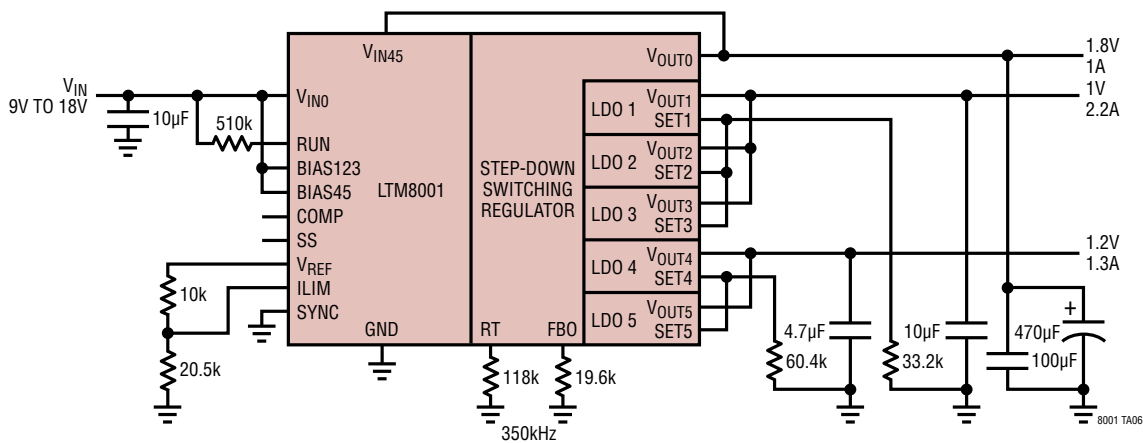
Three Output DC/DC μModule Converter
