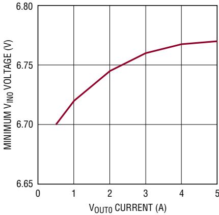
Minimum V_{IN0} vs Output Current, V_{OUT0} = 5\text{V}
