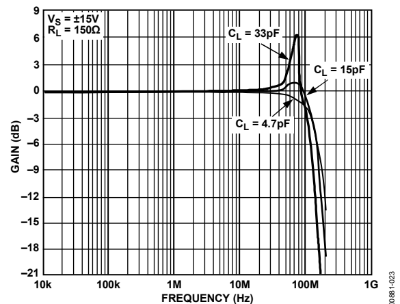
Figure 23. Closed-Loop Gain vs. Frequency vs. C_L , G = +1 , V_S = \pm 15V
