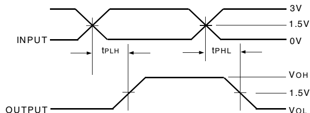
t_{SK(P)} = |t_{PHL} - t_{PLH}| Pulse Skew - t_{SK(P)}
