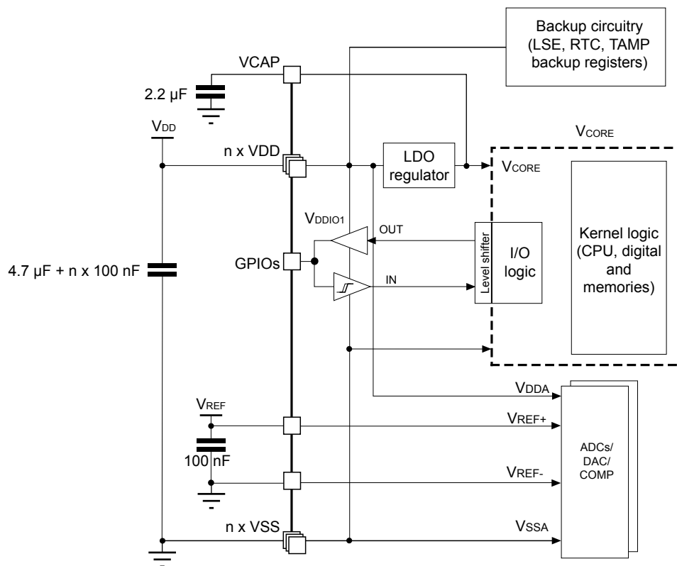
Figure 13. STM32C5A3xxx power supply scheme
