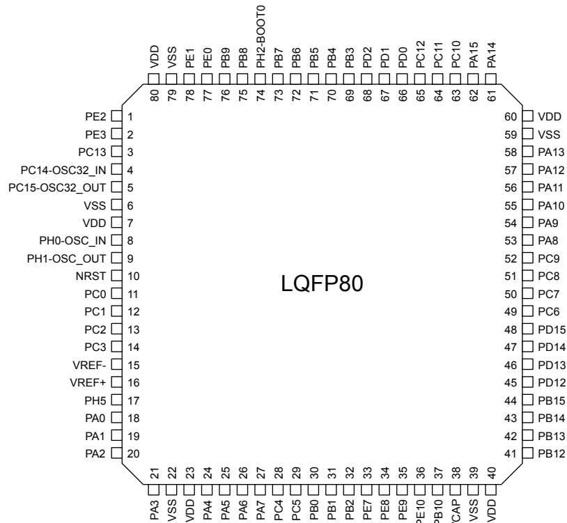
Figure 8. LQFP80 pinout
