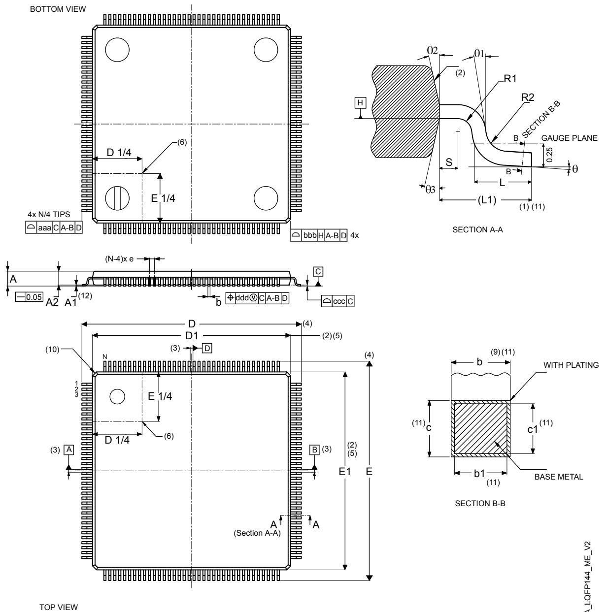
Figure 58. LQFP144 - Outline (15)
