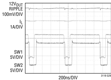
Switch and V_{OUT} Waveforms (12V IN , 12V OUT )
