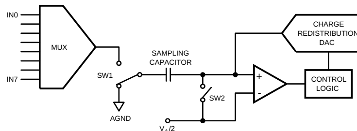
Figure 35. ADC088S052 in Hold Mode
