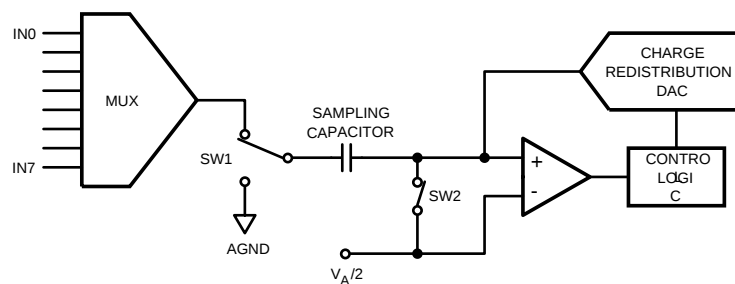
Figure 34. ADC088S052 in Track Mode
