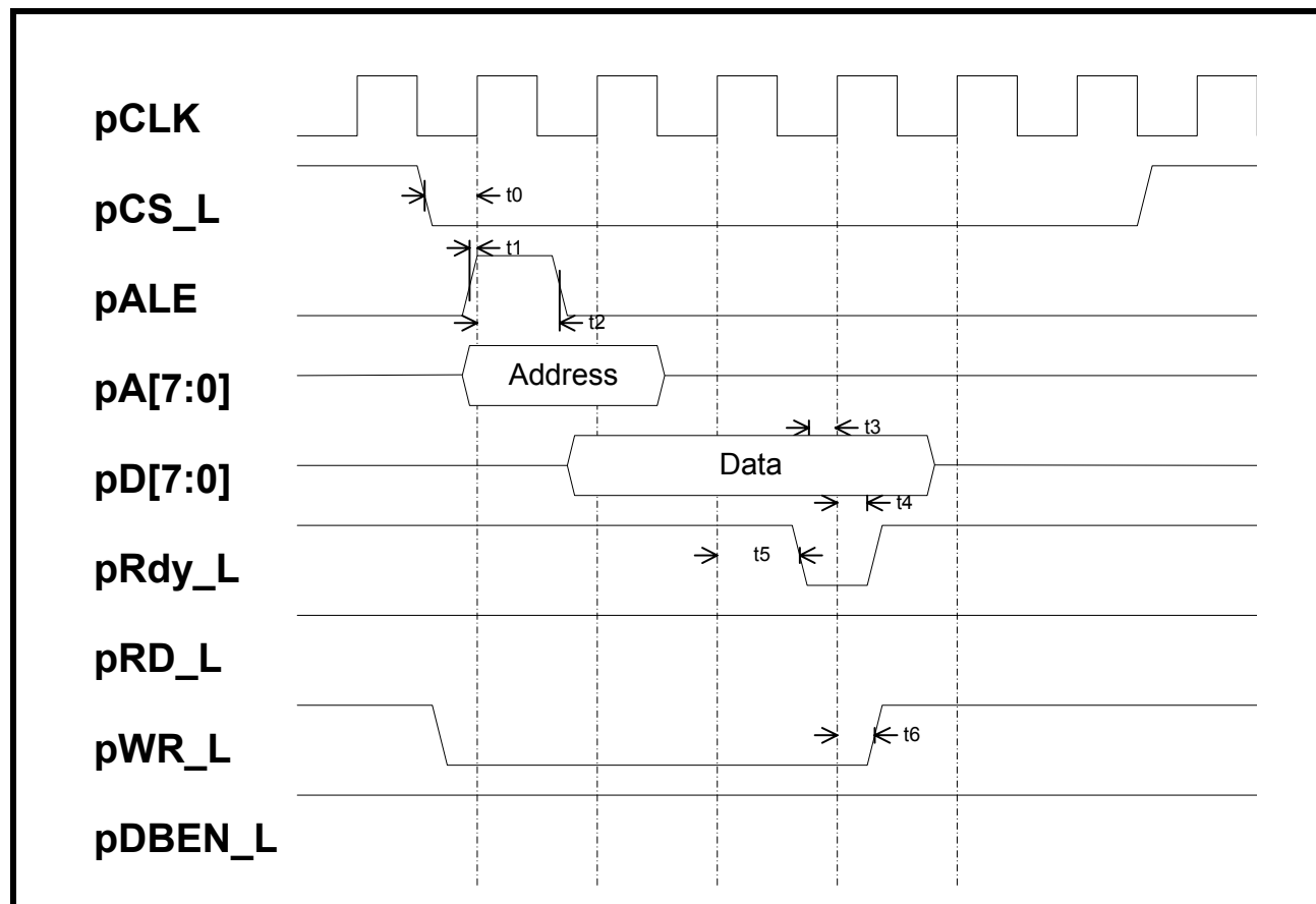
FIGURE 8. SYNCHRONOUS MODE 4 - IDT3051/52 INTERFACE TIMING (WRITE CYCLE)
