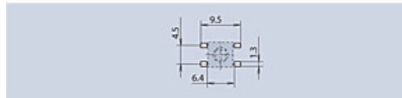
Layoutvorschlag · Layout Suggestion
