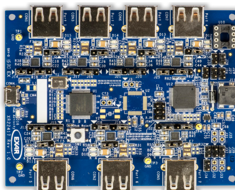
XR22417CV48EVB XR22417CV64EVB (Pictured)
