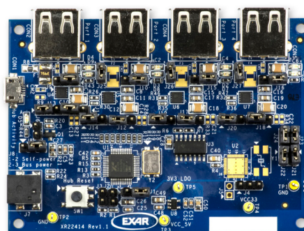
XR22414CL48EVB XR22414CV48EVB (Pictured)
