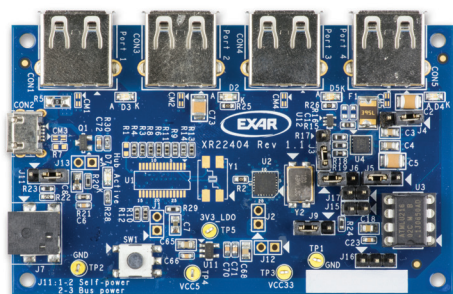
XR22404CG28EVB XR22404CL24EVB (Pictured)
