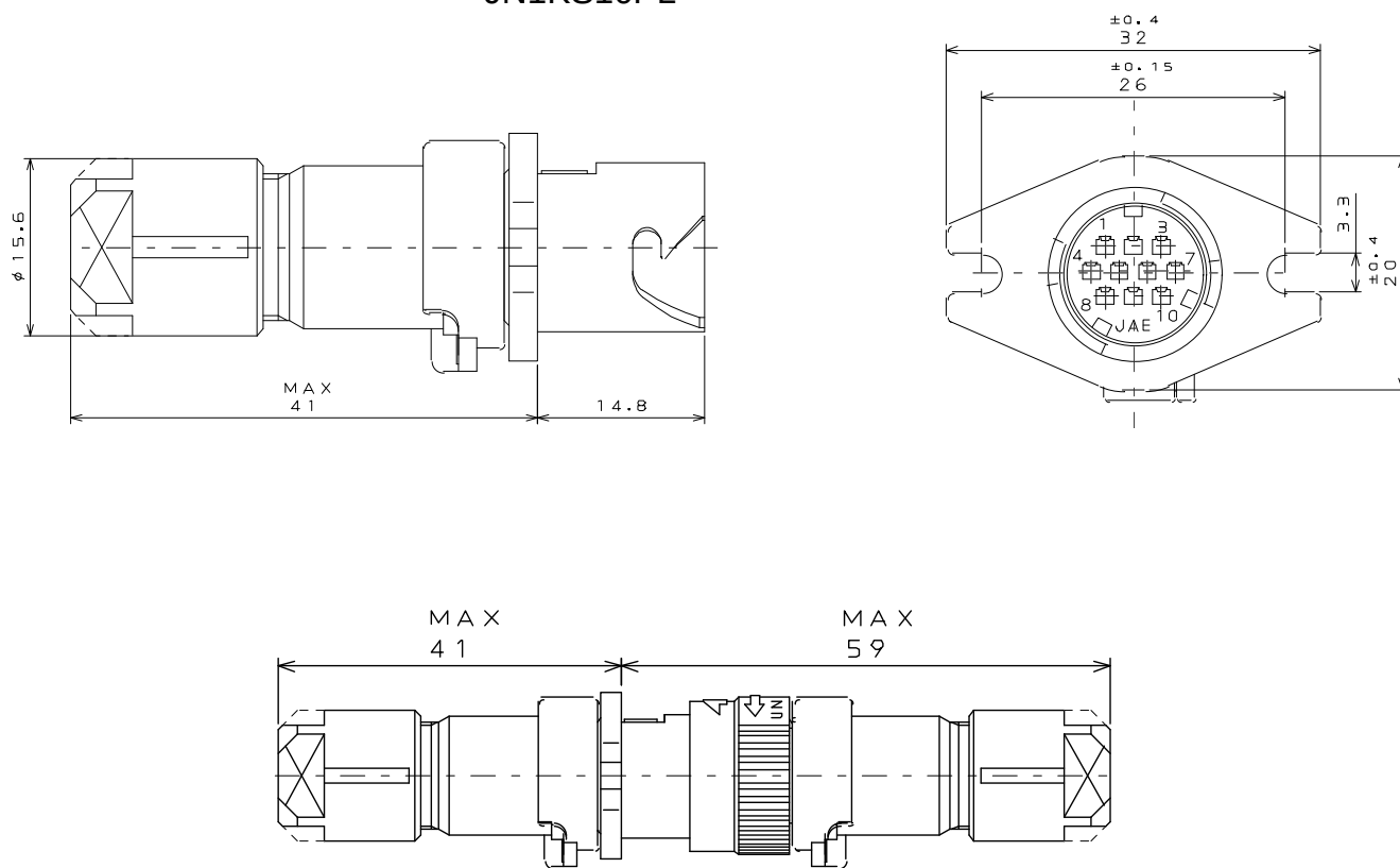
Drawing (when mated)
