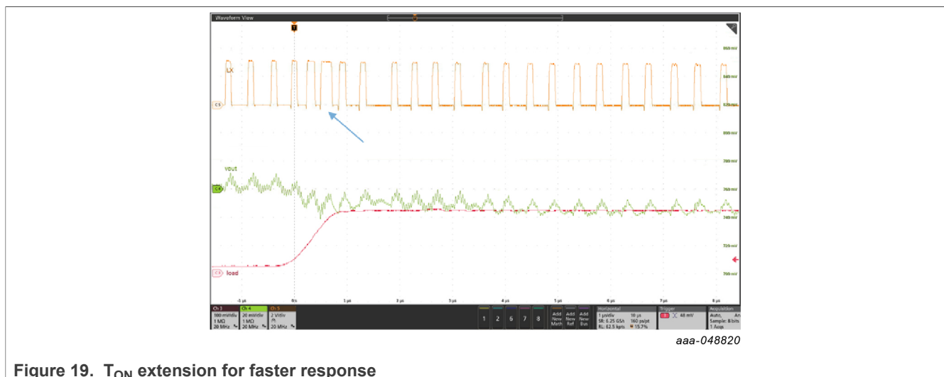
Figure 19. T ON extension for faster response
