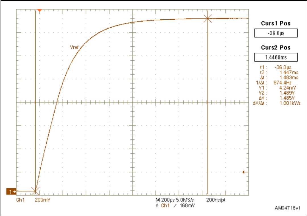
Figure 38. Reference startup, I_{REF} = 15\text{ }\mu\text{A} , T_A = 25\text{ }^{\circ}\text{C}
