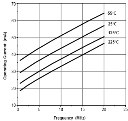
Operating current vs. frequency vs. temperature
