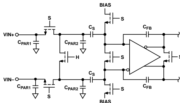
Figure 46. Switched-Capacitor Input
