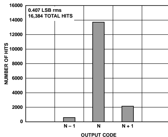
Figure 39. AD9634-250 Grounded Input Histogram, f_s = 250 MSPS
