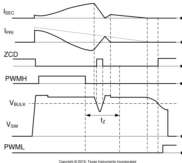
Figure 8-21. The Enhanced t_z Control for CCM Avoidance
