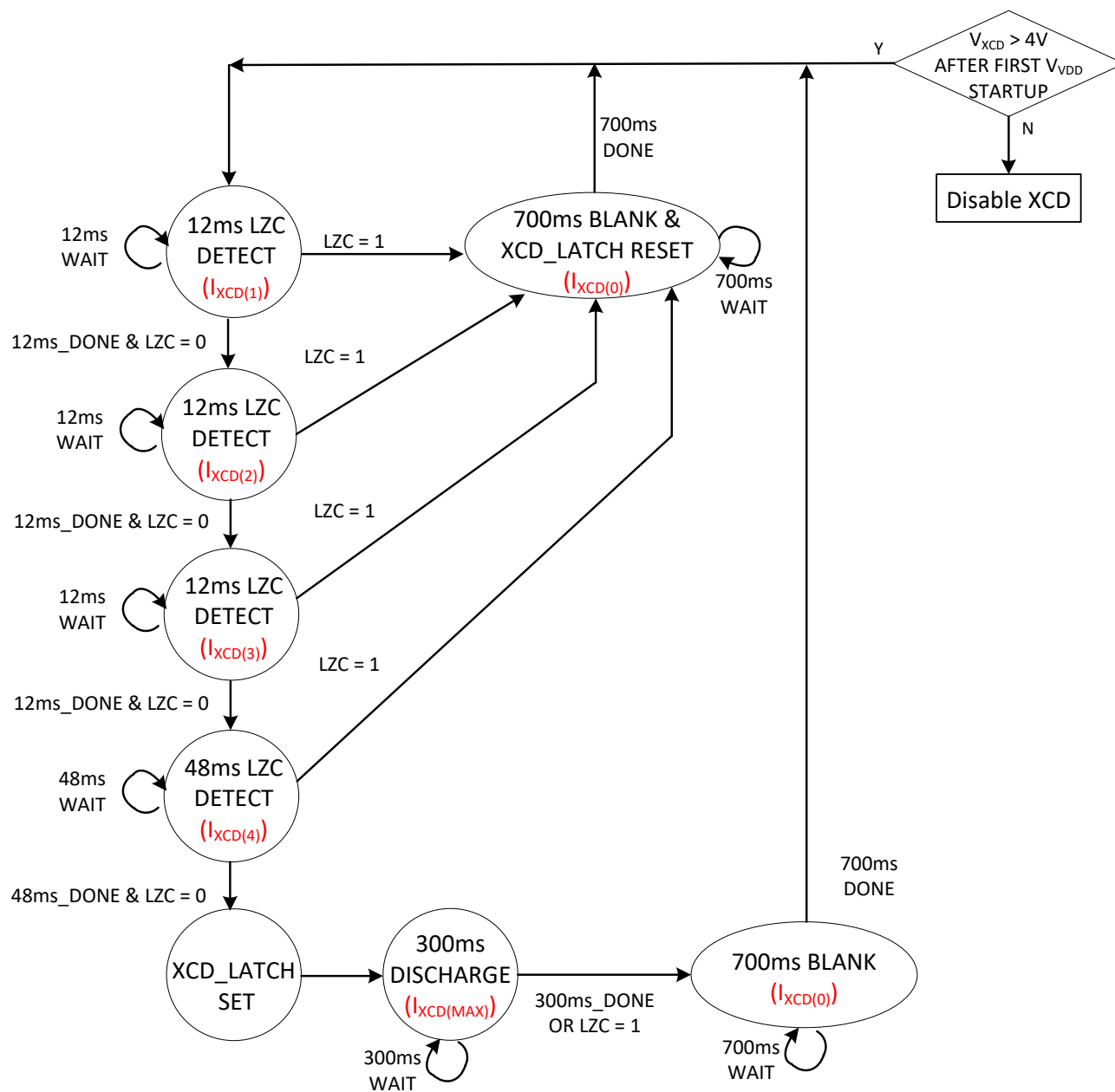
Figure 8-17. The State Diagram of the XCD-pin Function
