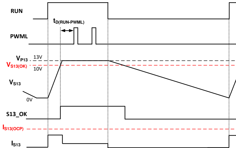
Figure 8-7. Power Management Function for a GaN Power IC and PFC Controller
