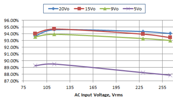
Figure 9-6. Full-Load Efficiency vs. Input Voltage
