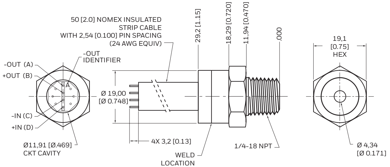
Figure 4. Package 5: 1/4-18 NPT
