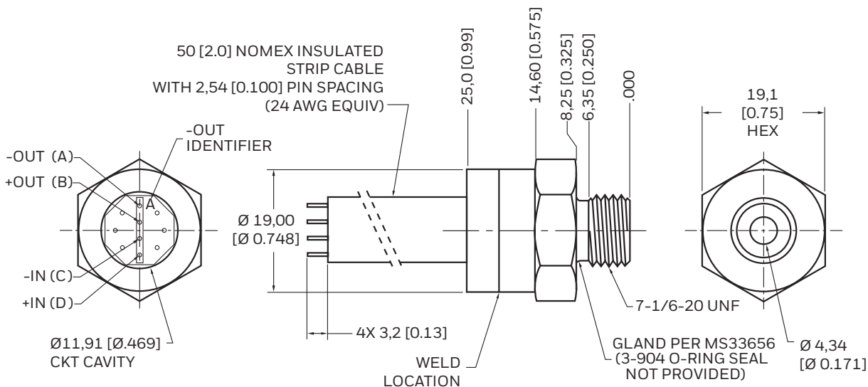
Figure 5. Package 6: 7/16-20 UNF
