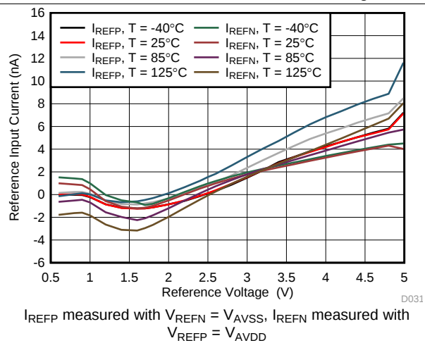
Figure 65. ADC2 Reference Input Current
