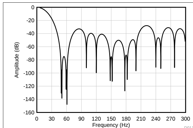
Figure 89. FIR Frequency Response (20 SPS)
