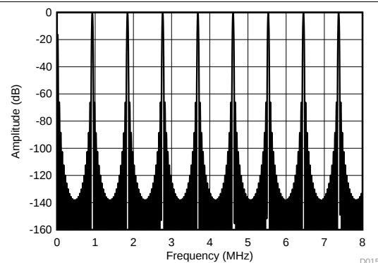
Figure 152. Frequency Response to 8 MHz (38400 SPS)
