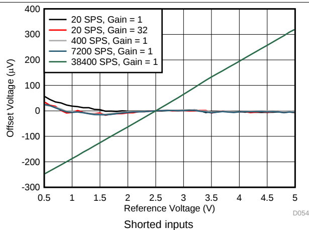
Figure 8. ADC1 Offset Voltage vs Reference Voltage
