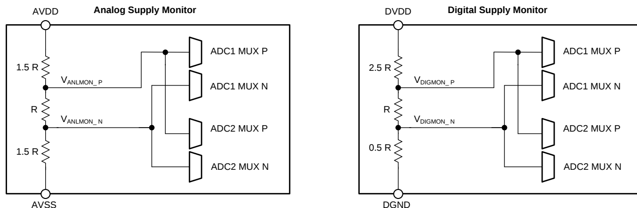
Figure 70. Power-Supply Monitors
