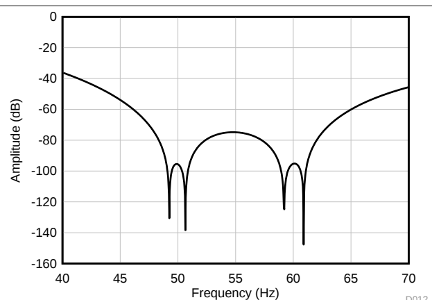
Figure 90. FIR Frequency Response Detail (20 SPS)
