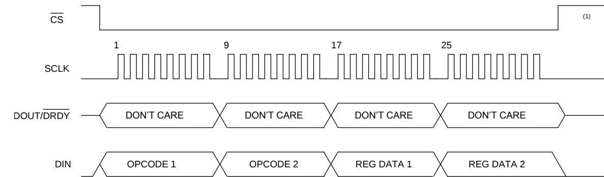
Figure 122. Write Register Sequence
