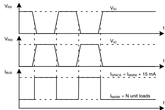
Figure 8. Output Waveforms
