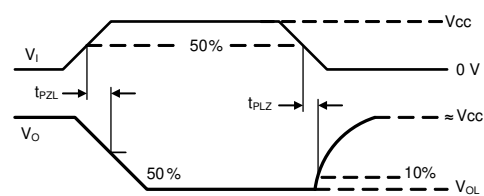
Figure 6-5. Measurement of Driver Enable and Disable Times With Active Low Output and Pull-up Load
