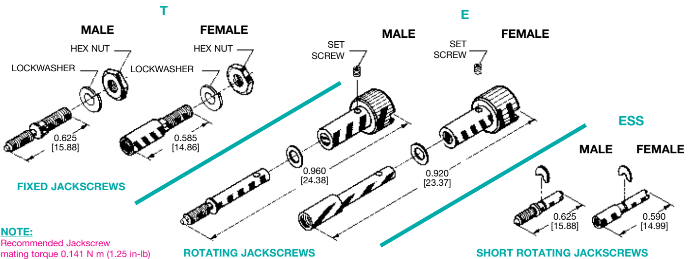
ROTATING JACKSCREWS
