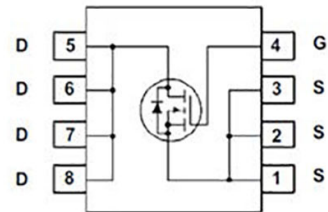
N-Channel MOSFET
