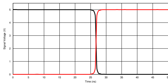
Figure 6-1. Response Time vs Output Voltage
