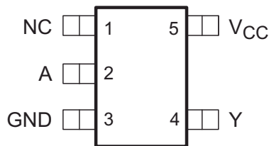
Figure 5-2. DCK Package 5-Pin SC70 Top View
