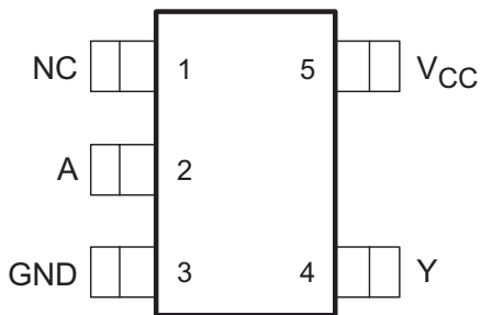
Figure 5-1. DBV Package 5-Pin SOT-23 Top View
