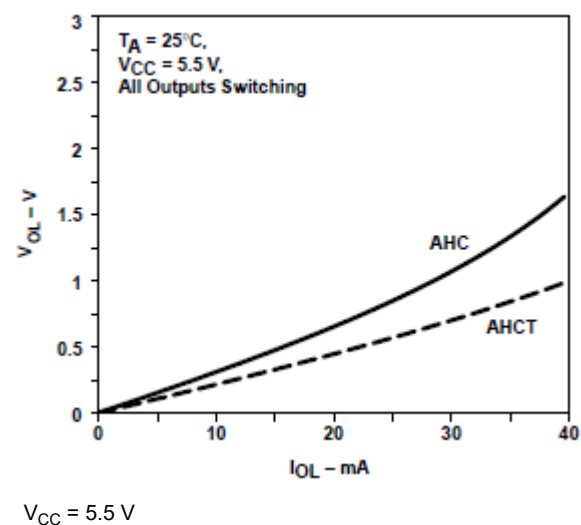
Figure 9-3. AHC Family V_{OL} vs I_{OL}
