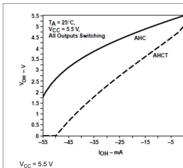
Figure 9-2. AHC Family V_{OH} vs I_{OH}
