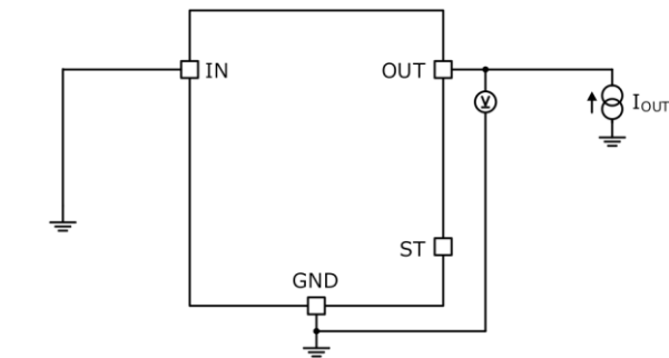
Measurement Circuit for Figure 8 and Figure 9
