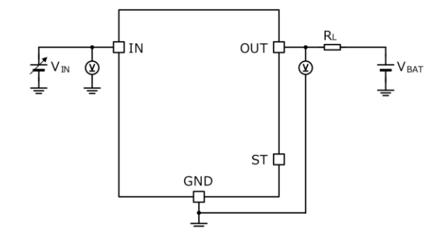
Measurement Circuit for Figure 2
