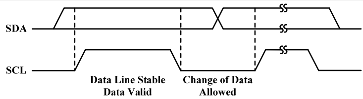
Figure 4 Bit Transfer
