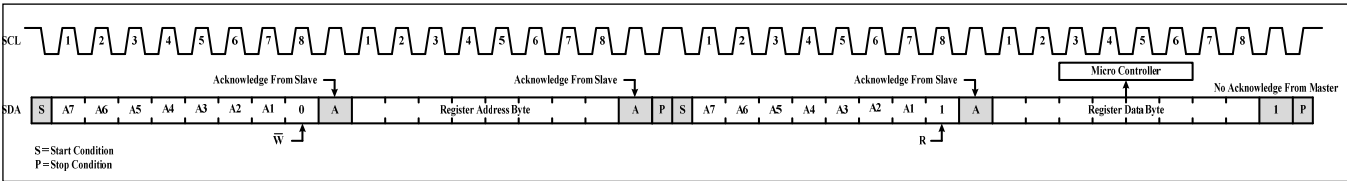
Figure 7 Reading from IS31FL3197
