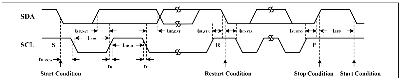
Figure 3 Interface Timing
