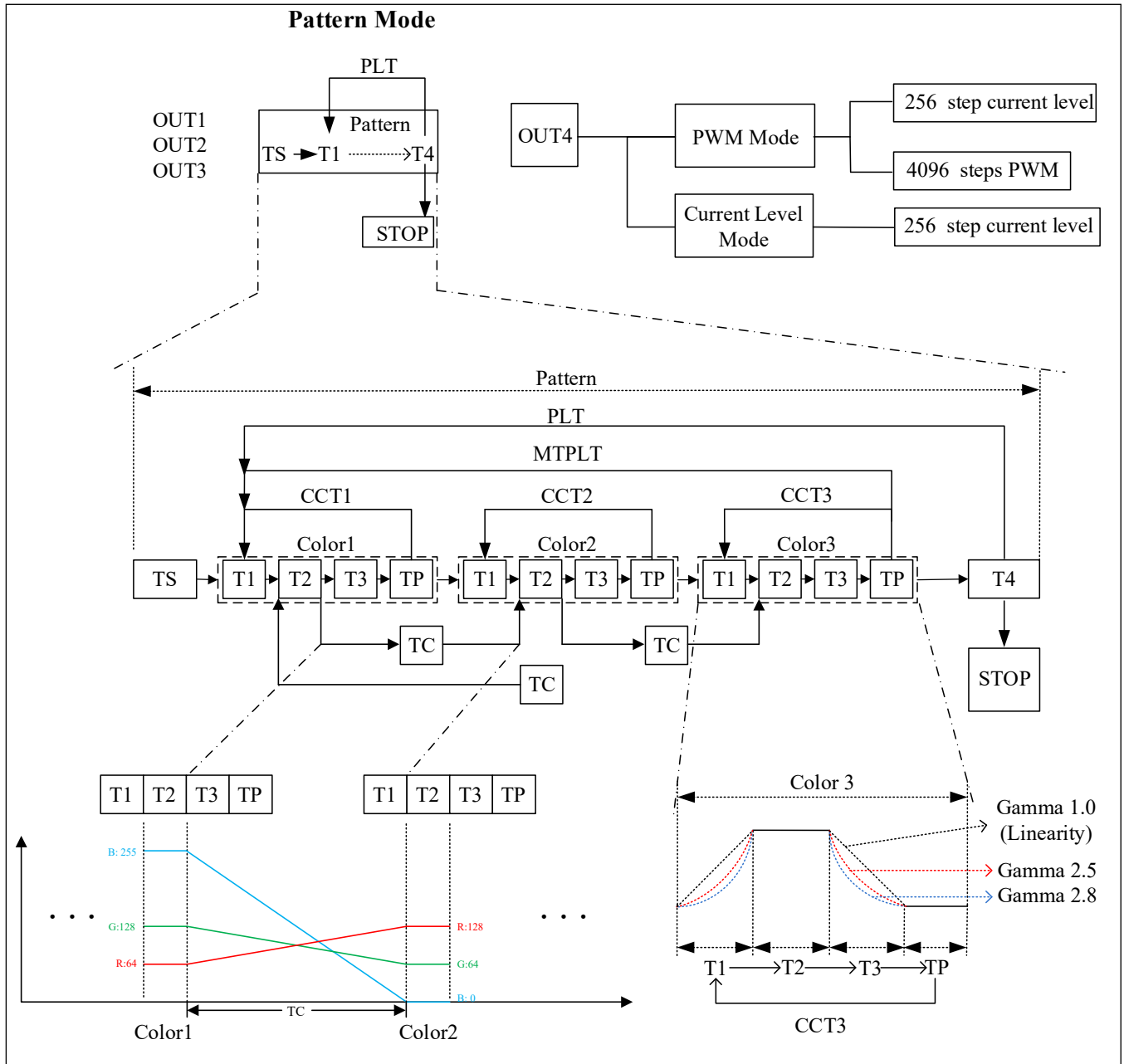
Figure 14 Pattern Mode
