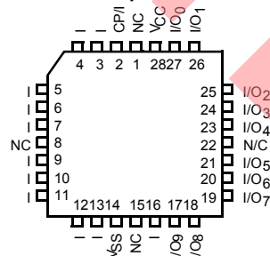
PLCC Top View
