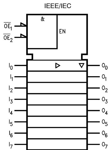
Figure 2. Logic Symbol
