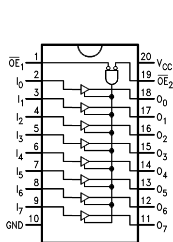
Figure 1. Connection Diagram
