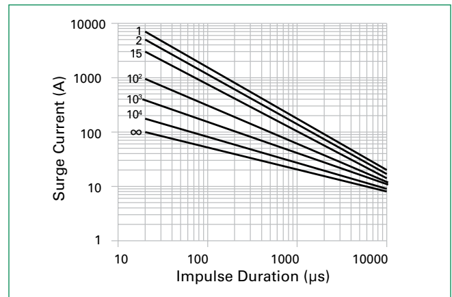
Repetitive Surge Capability for 14mm Parts
