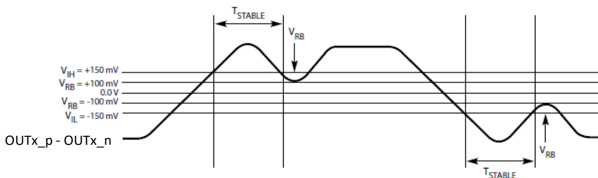
Figure 19. Differential Measurement Points for Ringback
