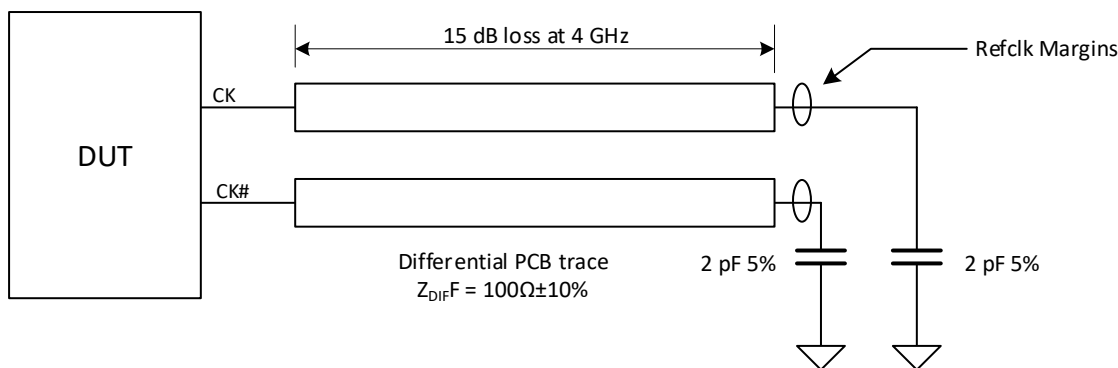
Figure 20. PCIe Test Circuit
