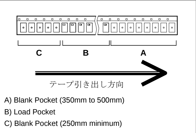
Fig.8 Taping
