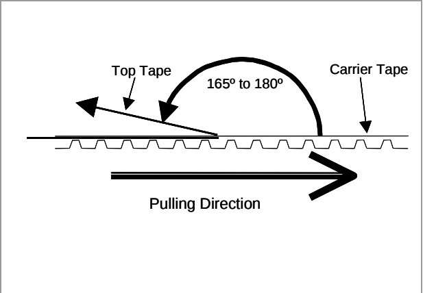
Fig.9 Peeling Strength
