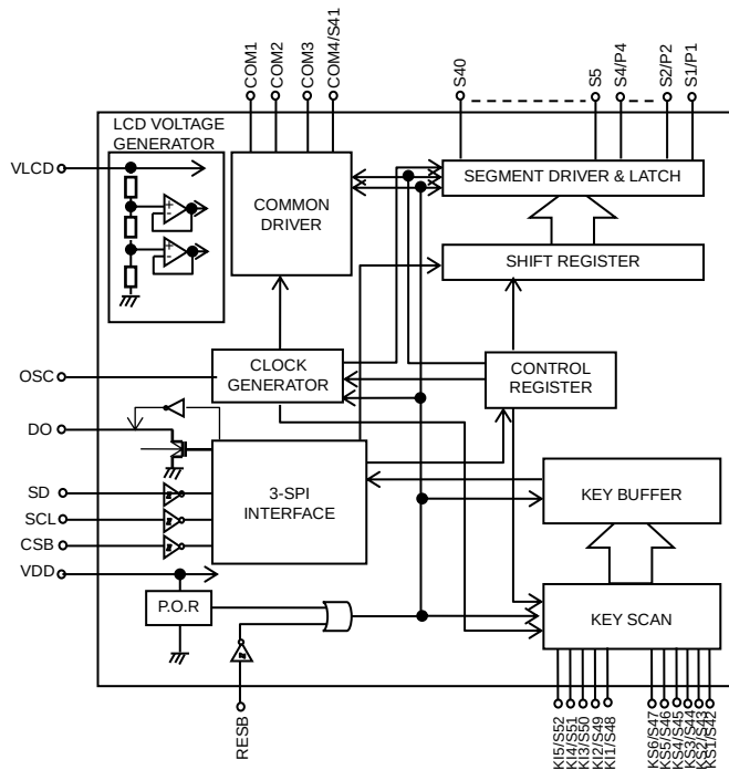
Figure 2. Block Diagram
