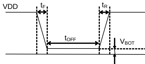
Figure 23. Power ON/OFF waveform
