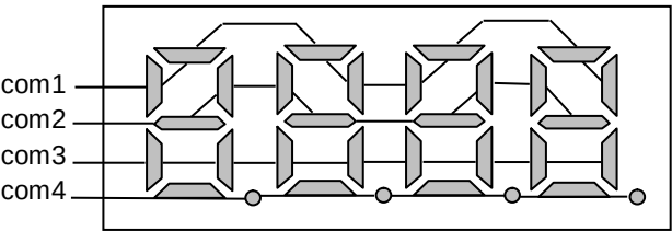
Figure 27. Example COM Line pattern
