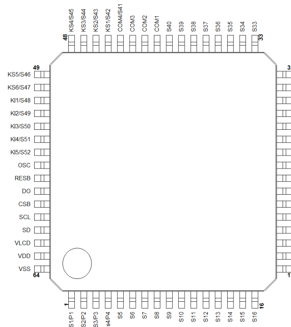
Figure 3. Pin Configuration (TOP VIEW)
