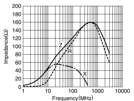
MZA3216Y600B
