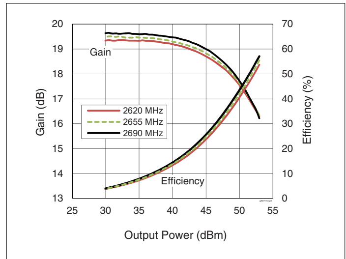
Figure 8. CW Performance
