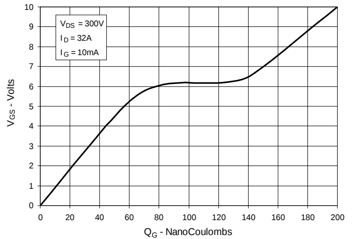
Fig. 7. Gate Charge
