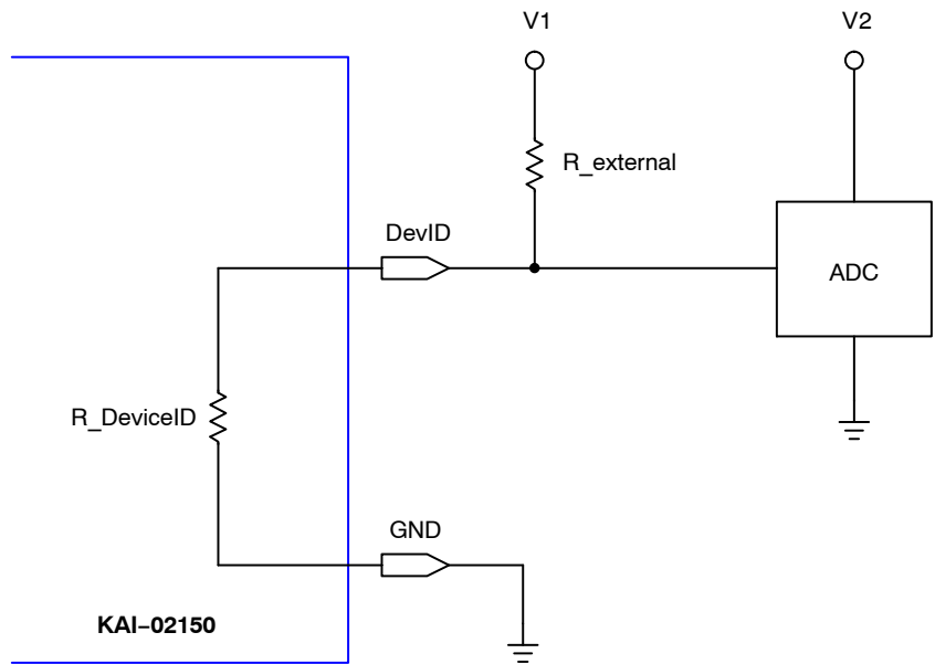
Figure 22. Device Identification Recommended Circuit
