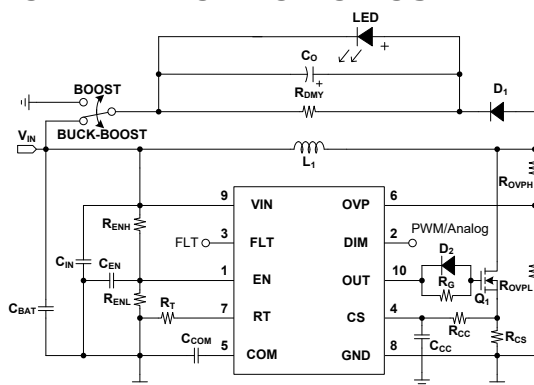
Buck-Boost Regulator
