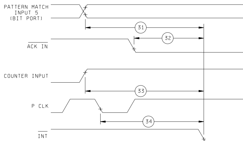
INTERRUPT TIMING
