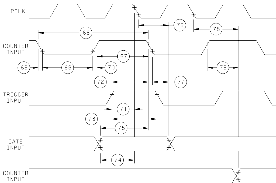
COUNTER/TIMER TIMING
