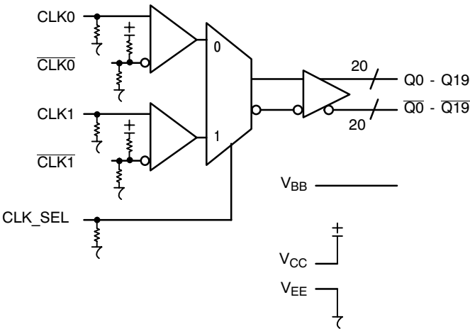
Figure 3. Logic Diagram
