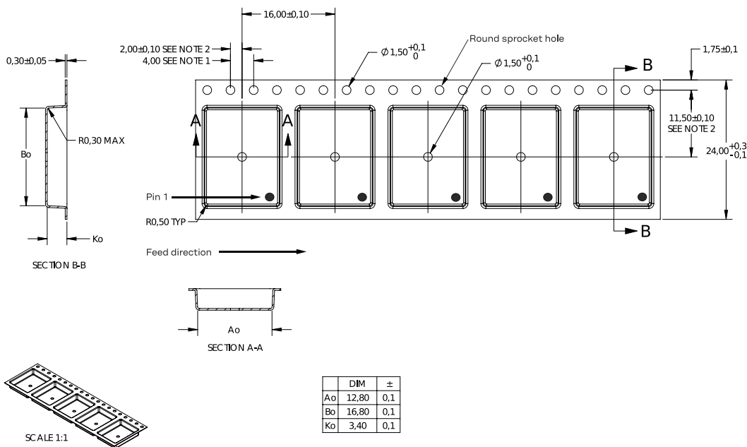
Figure 6: Feed direction, orientation, and dimensions (in mm) of NEO-M9V-20B modules on the tape
