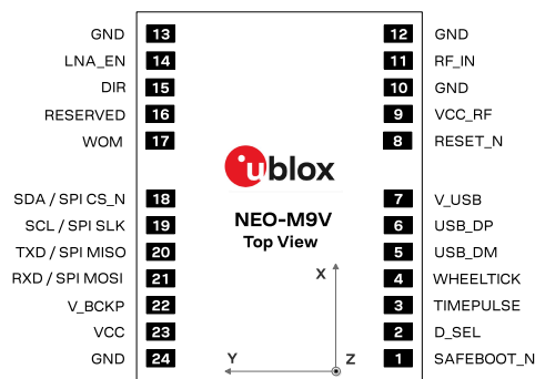
Figure 2: NEO-M9V-20B pin assignment
