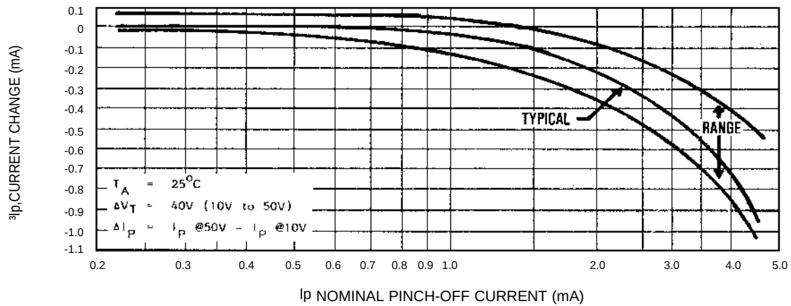
FIGURE 4 TEMPERATURE COEFFICIENT
