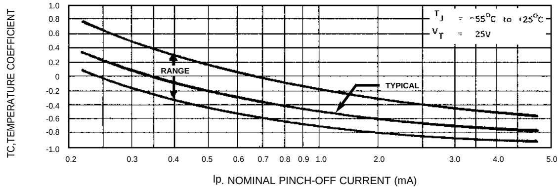
FIGURE 3 TEMPERATURE COEFFICIENT
