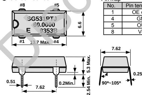
Pin map
