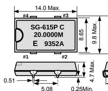
Pin map
