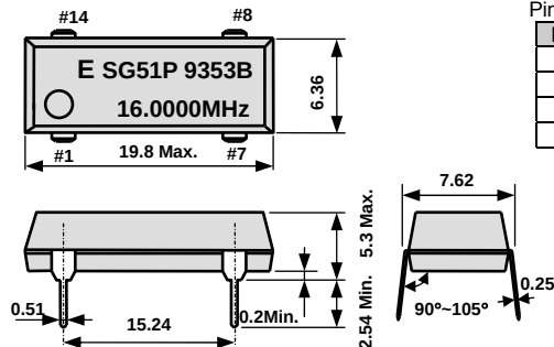
Pin map
