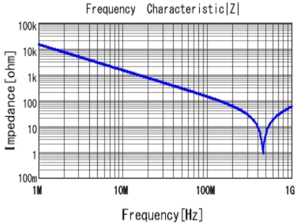
■ DE11XRA100KJ4BQ01F |Z| DC0V, 20degC
