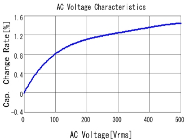
■ DE11XRA100KJ4BQ01F C-AC Voltage capchange, DC0V, 20.0
