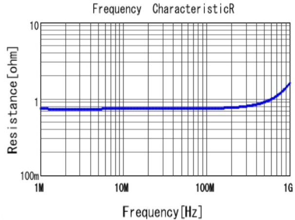
■ DE11XRA100KJ4BQ01F R DC0V, 20degC
