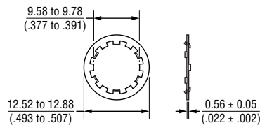
LOCKWASHER H-37-2
