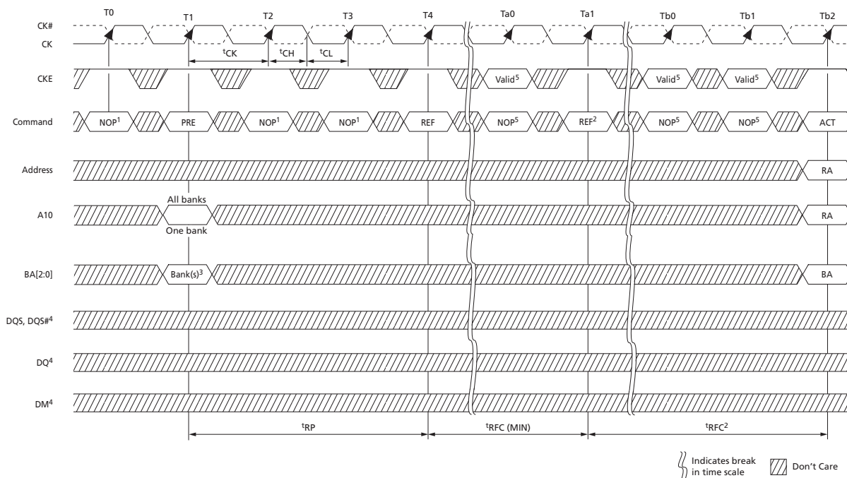
Figure 37: Refresh Mode
