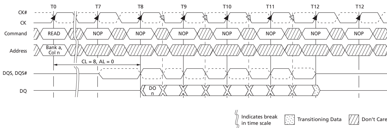
Figure 64: READ Latency
