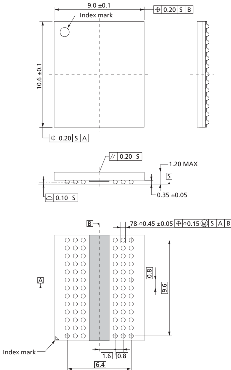
Figure 8: 78-Ball FBGA – x4, x8
