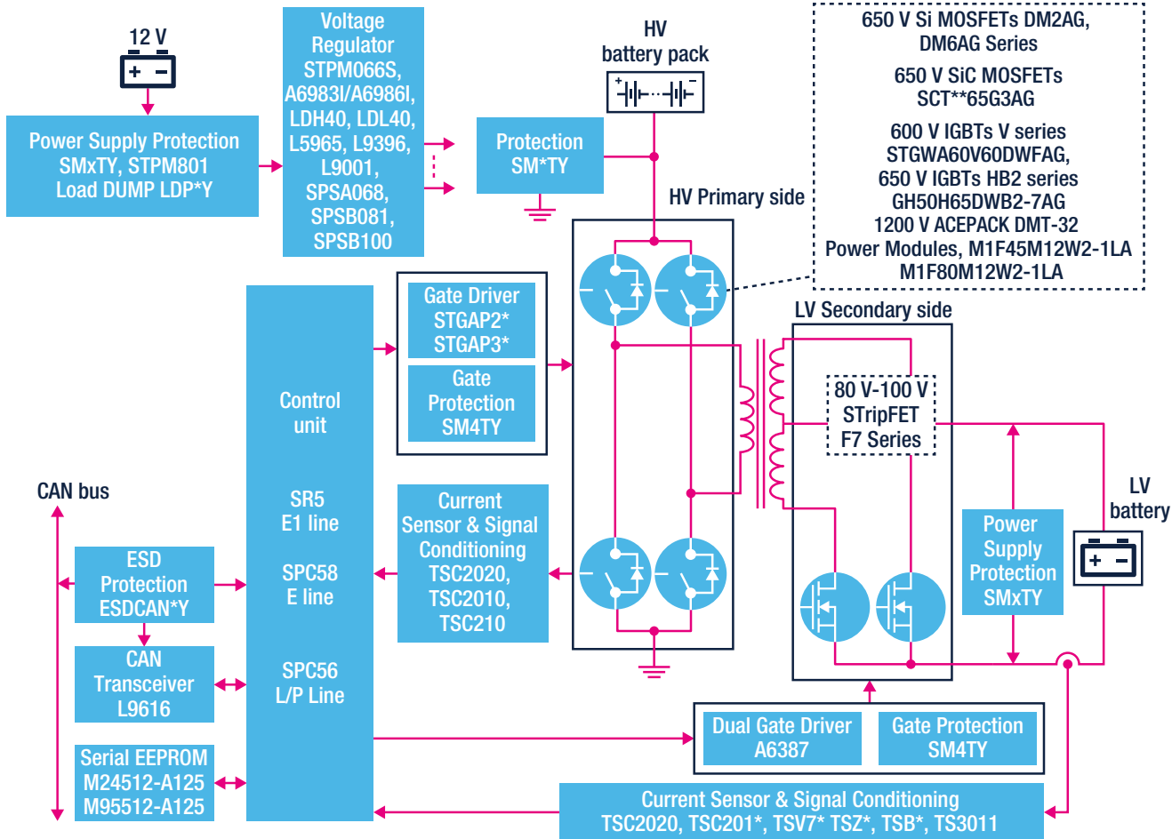
Typical block diagram - bidirectional DC-DC converter
