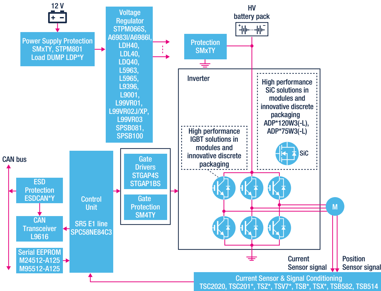
Typical block diagram - main inverter
