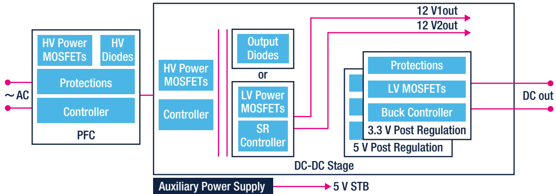
Typical configuration
