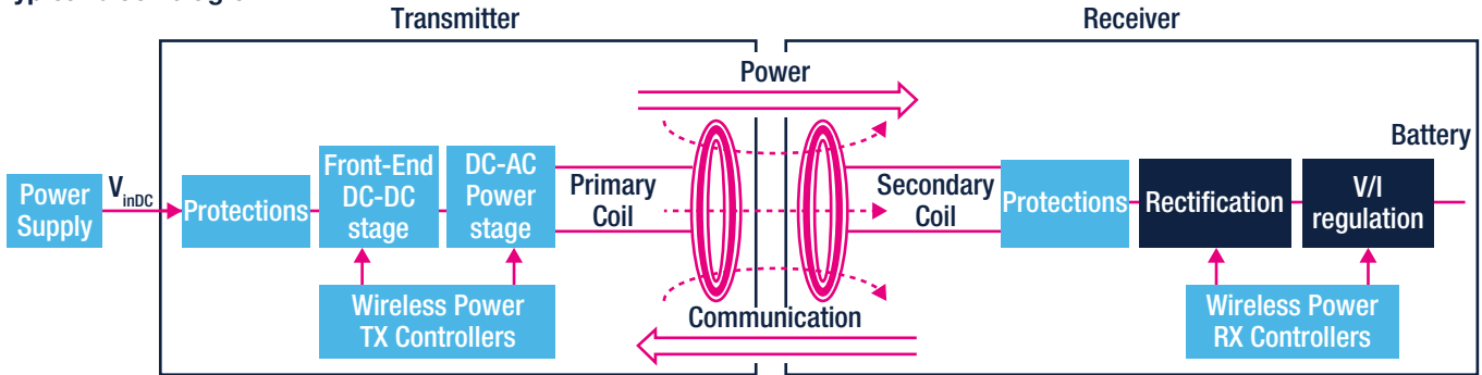
Typical block diagram
