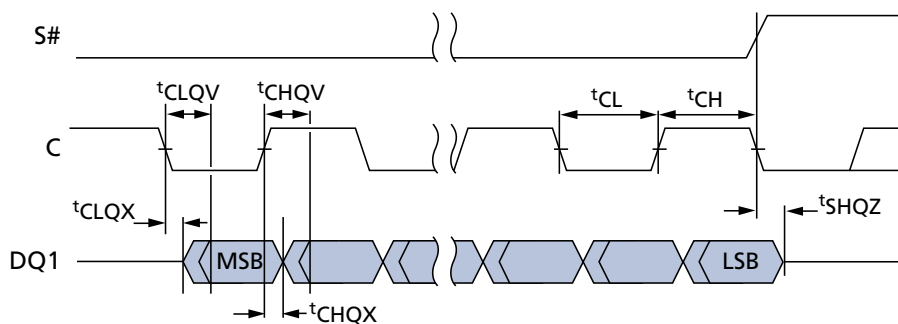
Figure 52: Output Timing for DTR
